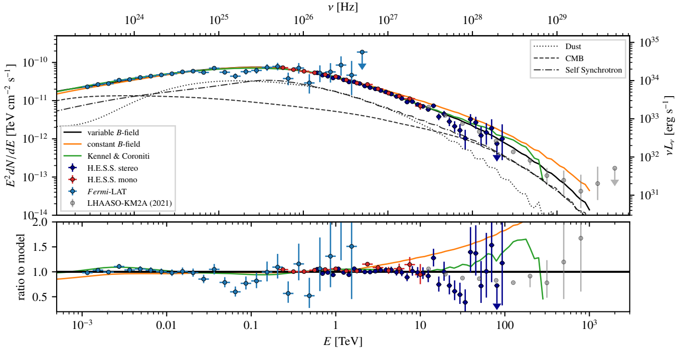
Fig. 12. IC flux predictions of the three models, together with the Fermi -LAT and H.E.S.S. flux points derived in this work. The LHAASO flux points, taken from Cao et al. (2021), are only shown for comparison. The dashed, dotted and dash-dotted lines show the individual contributions of seed photon fields for the variable B -field model. The bottom panel shows the ratio of the data points as well as the constant B -field and K&C model with respect to the variable B -field model.
