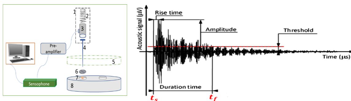
Fig. 1. Schematics of the setup (1: microphone housing, 2: pressing spring, 3: microphone, 4: steel waveguide, 5: Plexiglas, 6: silicon wafer, 7: sample, 8: DSC furnace) and a typical temporal shape of acoustic emission signal with the definition of the measured parameters. The duration time is the time at which the signal falls below the threshold (and is equal to t_f - t_s ). The threshold was determined far from the spin transition event, i.e. when no AE due to structural changes was present (see also the text).
