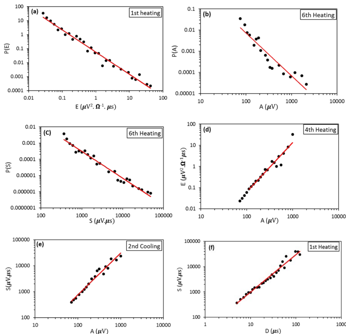
Fig. 5. Examples of probability distribution density functions of (a) energy, (b) amplitude and (c) area as well as illustrations of (d) energy-amplitude, (e) area-amplitude and (f) area-duration power relations for compound 1. The fitted straight lines are the results of fits according to eqn. (1) (see also the text and ESI) as well as of fits according to the power relations between E and A as well as S and A .
