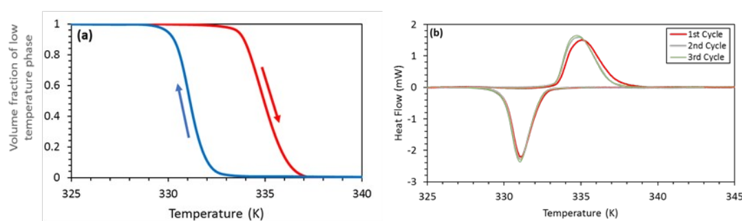
Fig. 2. Hysteresis loop (a) calculated from the DSC curves (b) for compound 1 .
