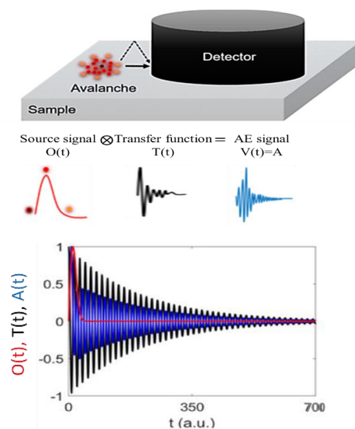
Fig. 6. Schematic representation of the composition of an avalanche signal in acoustic emission experiments. (Reprinted with permission from ref. 55.) During local switching, an avalanche with V(t) emits a strain signal (i.e. the source function) which propagates through the sample and is eventually measured by the detector. During the propagation and attenuation, the signal also generates the ringing of the sample. The profile of a source delta function would generate T(t) , the so-called transfer function. The distortion is manifested on the time scale in a long exponential decay tail at the end of the avalanche. Thus, the duration of the avalanche is heavily distorted, while the amplitude and rising time are less influenced.
