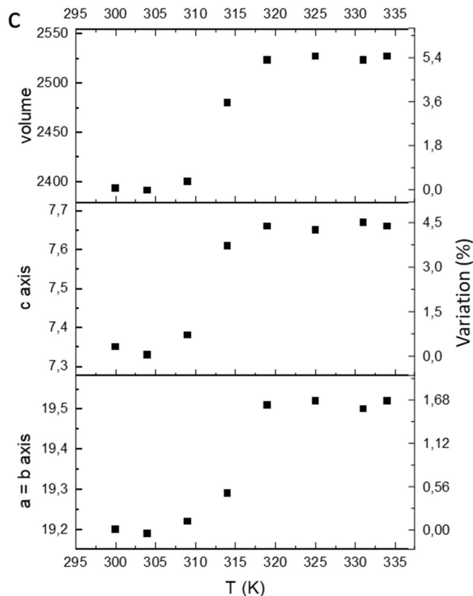
Fig. 4 Representative powder X-ray diffraction pattern in the LS and HS states (a), unit-cell parameters (b) and thermal variation of the unit cell parameters (c) of complex 3d.
