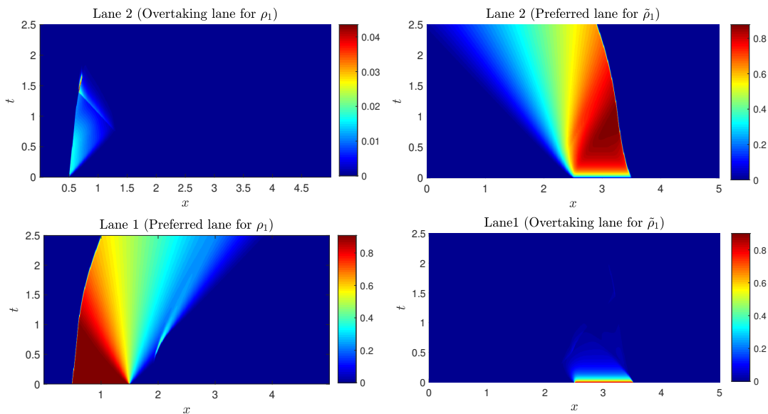
Figure 4. Example 2, heat map of \boldsymbol{\rho}^\Delta(\cdot, t) = [\rho_1(\cdot, t), \rho_2(\cdot, t)] and \tilde{\boldsymbol{\rho}}^\Delta(\cdot, t) = [\tilde{\rho}_1(\cdot, t), \tilde{\rho}_2(\cdot, t)] , t \in [0, 2.5] . Dynamics of numerical solution for (Left-top) \rho_2 (Left-Bottom) \rho_1 (Right-top) \tilde{\rho}_1 (Right-Bottom) \tilde{\rho}_2
