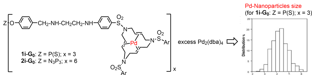
Scheme 9. Macrocycles on the surface of dendrimers, used for complexing palladium as discrete complexes or as palladium nanoparticles. Heck coupling reactions, and recycling.
