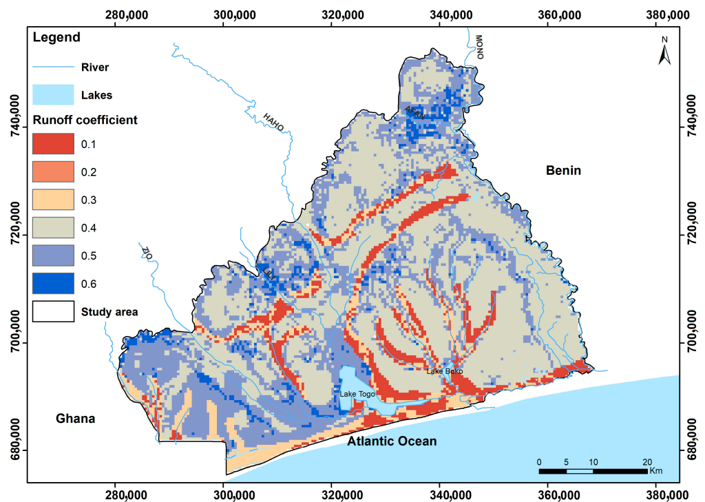
Figure 12. Runoff coefficient map.
