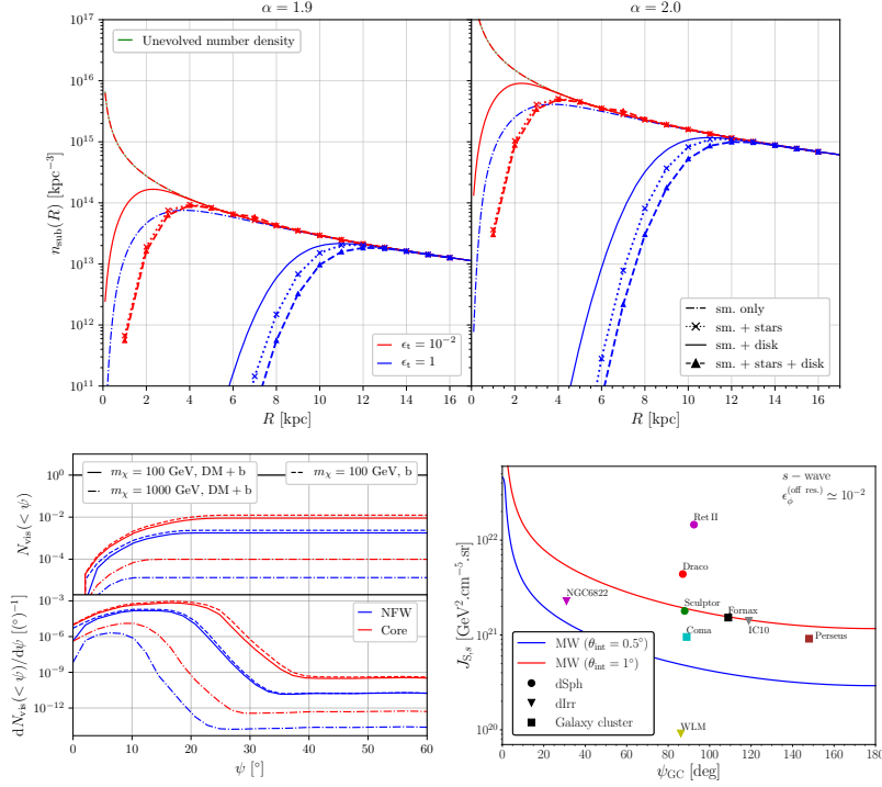
Figure 1: Top panels: subhalo number density profiles obtained for a constrained MW mass model, with the effect of different sources of tidal stripping (the smooth potential, disk shocking, and/or individual encounters with stars), showing the fragile vs. resilient model for tidal disruption (assuming simple power laws of index \alpha for the initial mass function); from [8]. Bottom left: angular distribution of subhalos potentially visible with Fermi-LAT for an observation time of 10 years, assuming an annihilation cross section at the limit of exclusion from the non-observation of the smooth halo (annihilation to \tau^+\tau^- is assumed); from [10]. Bottom right: classification of gamma-ray targets after including Sommerfeld-enhancement effects in an s -wave annihilating WIMP model and accounting for the presence of subhalos; from [11].
