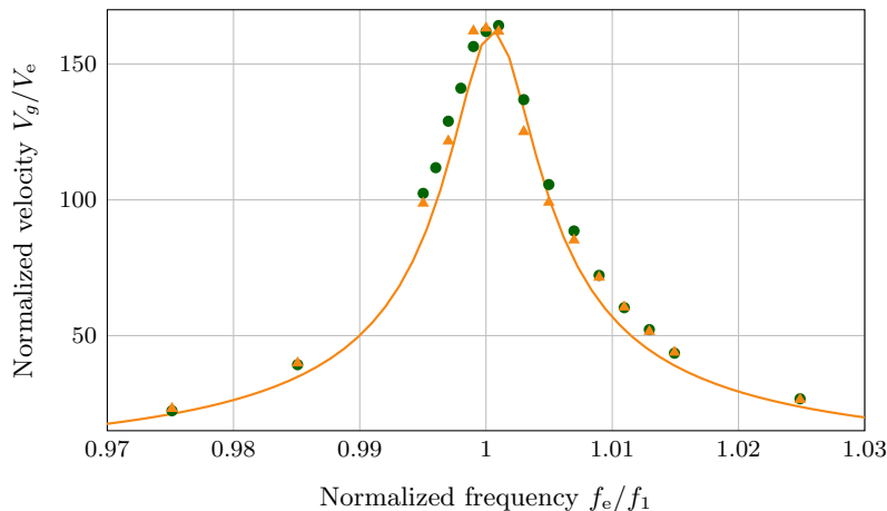
Figure 8: Non-perforated plate velocity normalized by base velocity around the first plate resonance frequency f_1 = 10.05 \text{ Hz} , for two base accelerations (experimental results are represented by points and the analytical result by a solid line): \gamma_e = 70 \text{ mm s}^{-2} ( \bullet ); \gamma_e = 90 \text{ mm s}^{-2} ( \blacktriangle ). Experimental results are obtained through the set-up presented in Figure 7.
