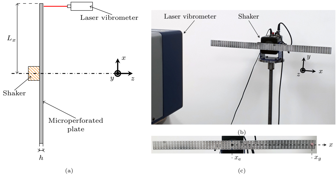
Figure 7: Experimental set-up and sample used for the frequency response of microperforated plate: (a) and (b) represent the experimental set-up respectively in the plan xz and xy ; (c) provides the microperforated sample investigated experimentally with x_e the abscissa of the excitation point and x_g the abscissa of the observation point. The MPP is made of aluminum and has a dimension of 560 \text{ mm} \times 30 \text{ mm} \times 1 \text{ mm} . The perforation parameters are set to d = 2.8 \text{ mm} and \phi = 10 \% .
