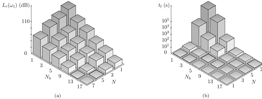
Figure 1: Influence of the number of harmonics on the forced response of the first mode of a simply supported microperforated plate. (a) normalized residual calculated from Equation (25) for F_{\text{ext}} = 0.1 \text{ N} ; (b) computation time (inverted axes for readability).
