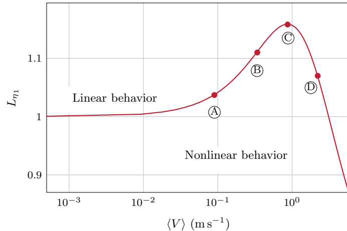
Figure 5: Normalized overall nonlinear loss factor as a function of the forcing amplitude. The microperforated plate is simply-supported, and the parameters for the perforations are d = 2.2 \text{ mm} and \phi = 10\% . The Forchheimer parameter is determined using Equation (9), resulting in \xi = 0.87 \text{ s m}^{-1} . The excitation amplitudes of points A, B, C and D as well as their corresponding coordinates are listed in Table 1.
