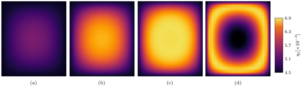
Figure 6: Spatial distribution of the loss factor \eta_1(\omega_1, V(x, y)) on the plate, obtained from Equation (28) at the first resonance frequency \omega_1 for the four excitation points listed in Table 1 and shown in Figure 5: (a) Excitation Ⓐ corresponding to F_{\text{ext}} = 0.02 N; (b) Excitation Ⓑ corresponding to F_{\text{ext}} = 0.08 N; (c) Excitation Ⓒ corresponding to F_{\text{ext}} = 0.20 N; (d) Excitation Ⓓ corresponding to F_{\text{ext}} = 0.55 N.
