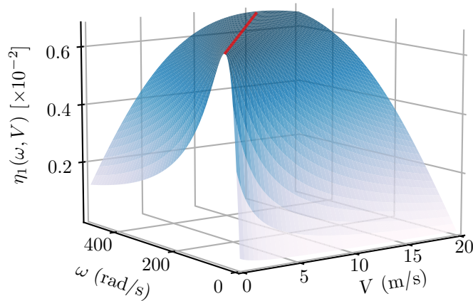
Figure 3: Loss factor \eta_1 as a function of the angular frequency \omega and the magnitude of the relative fluid-solid velocity V . The solid line (—) corresponds to the maximum of \eta_1 . The simply-supported MPP has dimensions 490 \text{ mm} \times 570 \text{ mm} \times 1 \text{ mm} , along with a perforation ratio \phi = 10\% , a perforation diameter d = 2.2 \text{ mm} , and a Forchheimer parameter \xi = 0.87 \text{ s m}^{-1} .
