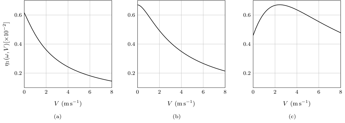
Figure 4: Loss factor obtained by Equation (28) of the first mode of the simply-supported aluminum MPP of dimension 490 \text{ mm} \times 570 \text{ mm} \times 1 \text{ mm} with \phi = 10\% and d = 2.2 \text{ mm} . The linear characteristic frequency \omega_c = 45 \text{ rad s}^{-1} is obtained from Equation (6). Three cases are presented: (a) \omega < \omega_c with \omega = 30 \text{ rad s}^{-1} ; (b) \omega = \omega_c and (c) \omega > \omega_c with \omega = 115 \text{ rad s}^{-1} . The Forchheimer parameter is calculated from Equation (9).
