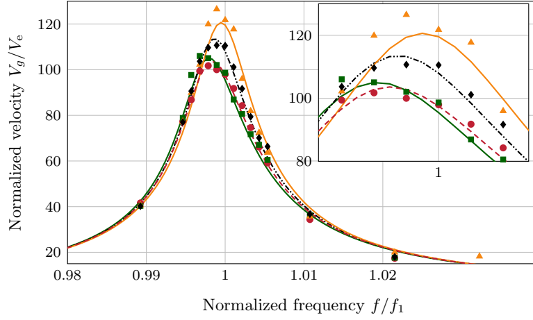
Figure 9: Microperforated plate velocity normalized by base velocity around the first plate resonance frequency f_1 = 9.28 Hz, for four base accelerations (experimental results shown by points and corresponding analytical results shown by solid or dotted lines): \gamma_e = 10 \text{ mm s}^{-2} ( \blacktriangle ); \gamma_e = 45 \text{ mm s}^{-2} ( \blacklozenge ); \gamma_e = 60 \text{ mm s}^{-2} ( \bullet ); \gamma_e = 80 \text{ mm s}^{-2} ( \blacksquare ). Experimental results obtained through the set-up presented in Figure 7 and solving Equation (37) with \xi = 1.43 \text{ s m}^{-1} . The perforation ratio is \phi = 10\% and the perforation diameter d = 2.8 \text{ mm} is chosen to have f_1 > f_c .
