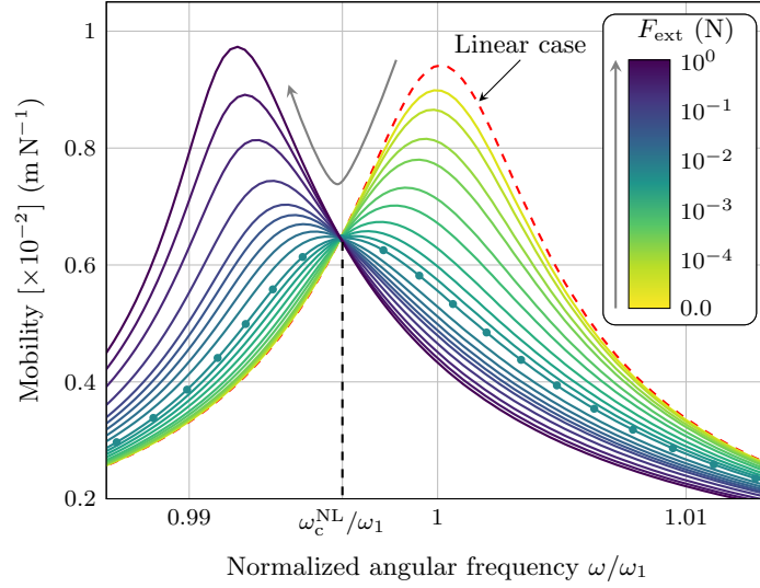
Figure 2: Mobility at the center of the simply-supported MPP for different amplitudes of the external force with d = 2.2 mm and \phi = 10\% . The mobility is given for F_{\text{ext}} \in [10^{-4}; 1] N and for: (---) F_{\text{ext}} = 10^{-4} N that corresponds to the linear case; (—●—) F_{\text{ext}} = 0.2 N which corresponds to the case where the maximum of the normalized displacement passes through a minimum. The \xi -parameter is obtained from Equation (9). The resolution procedure is performed for N = N_h = 1 .
