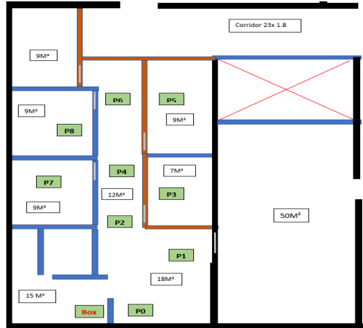
Fig. 1. Measurement apartment in Orange Labs Belfort.
