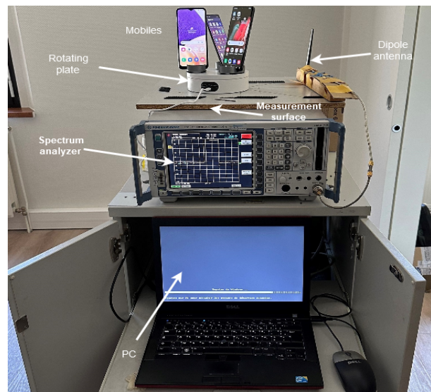
Fig. 2. Measurement setup.
