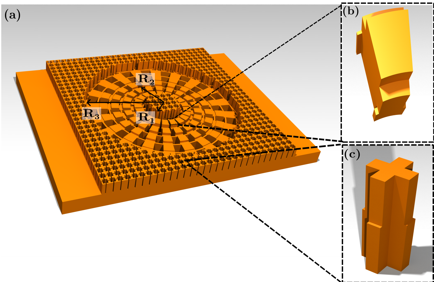
Fig. 4. (a) 3D thermal concentrator design. Note that the radius R_2 corresponds to a radius in the homogenous isotropic material which is mapped into the radius R_1 in this design
