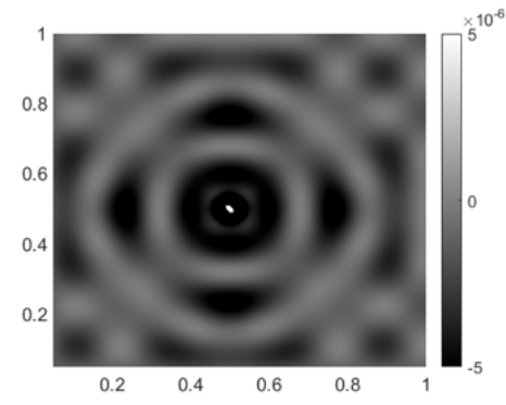
(d) Divergence of the irrotational intensity field at 1000 Hz
