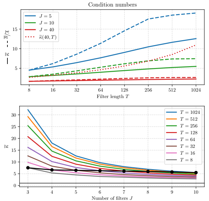
Fig. 4. We denote by \bar{A}, \bar{B} , and \bar{\kappa} the empirical means of the respective quantities over 1000 instances of \Phi with \sigma^2 = (JT)^{-1} . Top: Comparison of \bar{\kappa} (solid) and \bar{B}/\bar{A} (dashed) for increasing filter length T and different values of J . Bottom: Empirical mean \bar{\kappa} for increasing numbers of filters J and different values T . For J = \log_2 T (solid black), \bar{\kappa} remains approximately constant.
