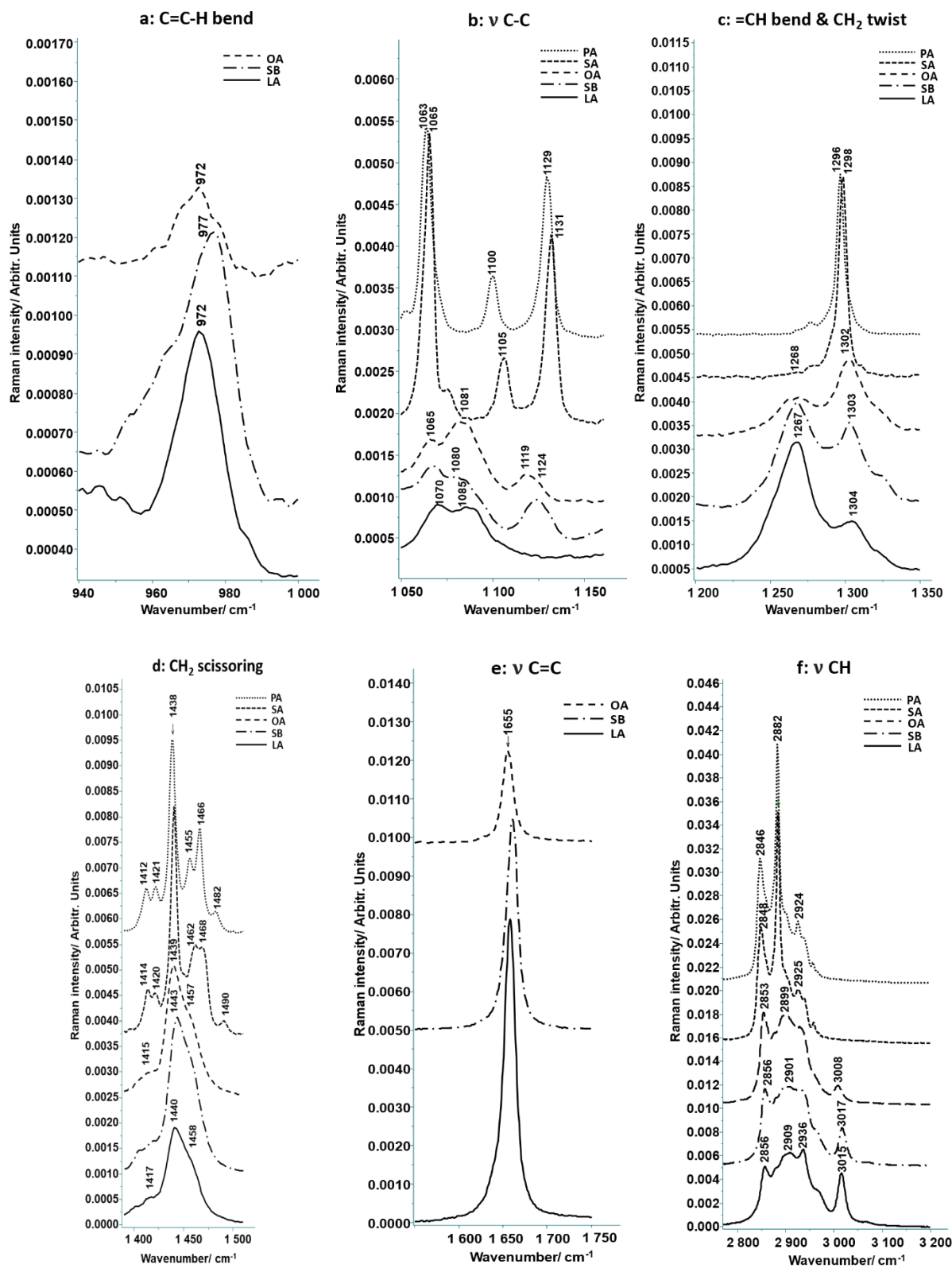
FIGURE 1 (A–F) Raman spectra of palmitic acid (PA), stearic acid (SA), oleic acid (OA), sebaleic acid (SB), and linolenic acid (LA) before UV irradiation. (A) C C H bend; (B) \nu C C; (C) CH bend and CH 2 twist; (D) CH 2 scissoring; (E) \nu C C; (F) \nu CH
