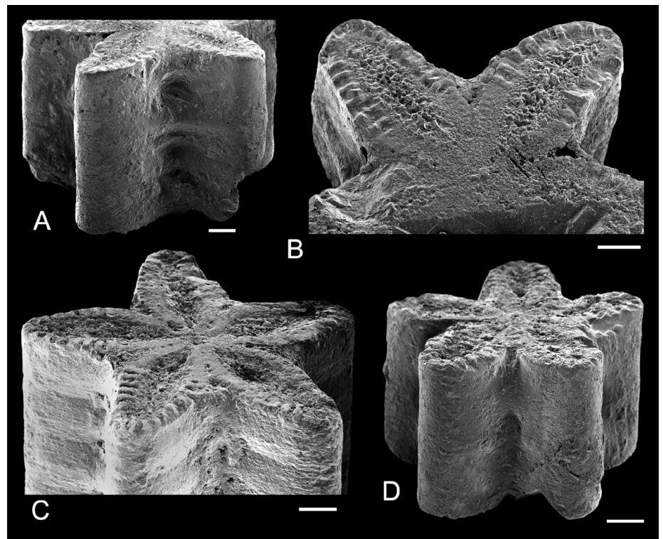
Fig. 8 - Columnal symplexes in Isselocrinus baldoensis n. sp. from Cambrigar; A-B) proximal pluricolumnal, paratype MGP-PD 1313R; A: side oblique view; B: articular facet. C) distal pluricolumnal, paratype MGP-PD 1312R, side oblique view. D) middle stalk pluricolumnal, paratype MGP-PD 1324R, side oblique view. Scale bars equal 1 mm.
