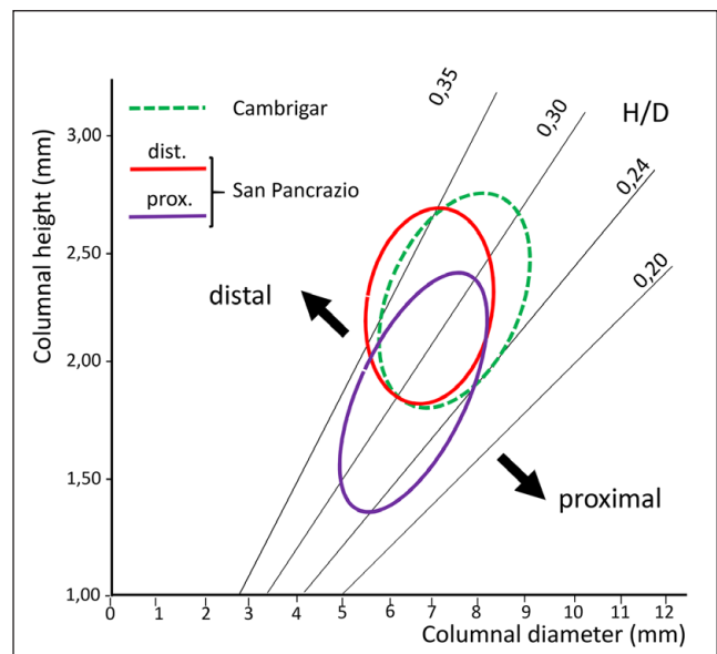
Fig. 11 - Columnal height and diameter values of Isselocrinus diaboli from San Pancrazio plotted in a bivariate graph and compared to results from Cambrigar columnals of the same species. Envelopes of points corresponding to the mean value in stalk fragments and pluricolumnals. See text for explanation.
