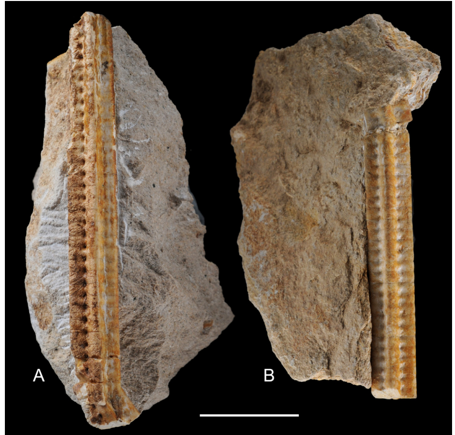
Fig. 7 - Isselocrinus baldoensis n. sp., two stalk fragments of morphotype A from Cambrigar; A) proximal fragment with conspicuous interarticular pores, paratype MGP-PD 1308R. B) proximal middle stalk fragment, holotype MGP-PD 1307R. Scale bar equals 20 mm.
