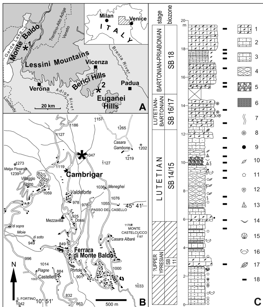
Fig. 1 - A) General map with the location of the Isellicrinus sites studied (asterisks): 1, Ferrara di Monte Baldo/Cambrigar; 2, Mossano/San Pancrazio; B) detailed map of the area north of Ferrara di Monte Baldo (Verona) with the location of the Eocene section of Cambrigar (asterisk); C) stratigraphic log of the "upper Cambrigar section", larger benthic foraminiferal biozonation (SB) according to Serra-Kiel et al. (1998). Legend: 1, larger foraminiferal calcirudites, locally glauconitic; 2, calcarenites, locally glauconitic; 3, marly calcarenites, locally glauconitic; 4, subnodular marly calcarenites; 5, synsedimentary fossiliferous breccia with calcarenitic clasts; 6, calcarenitic marls; 7, bioturbation; 8, calcareous algae; 9, iron sulfide nodules; 10, larger foraminifera; 11, crinoids; 12, echinoids; 13, gastropods; 14, ostreids; 15, undetermined bivalves; 16, crabs; 17, plant remains; 18, samples studied for larger foraminifera analysis.
