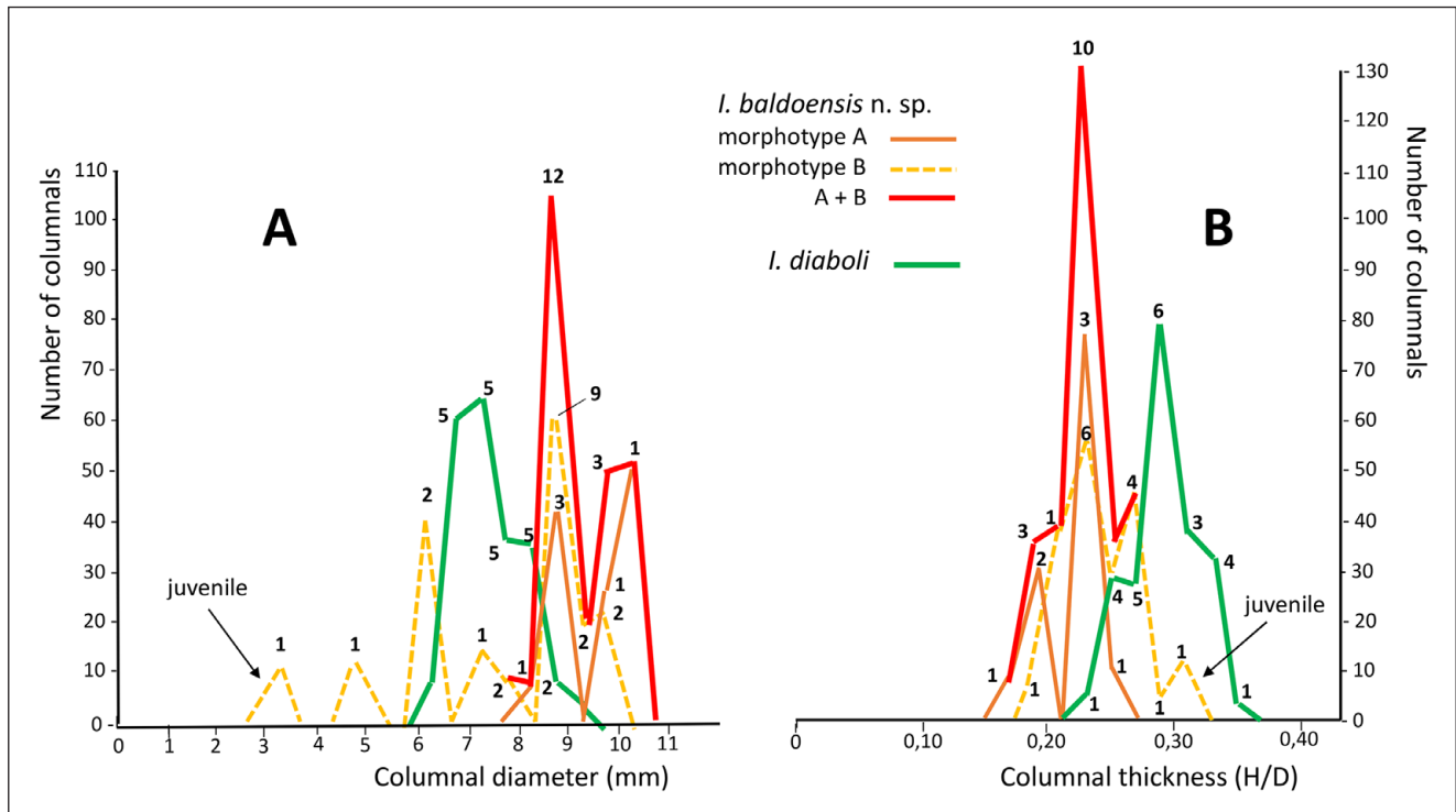
Fig. 10 - Frequency distribution of diameter (A) and thickness (B) in Isselocrinus columnals from Cambrigar. Small numbers: number of stalk fragments and pluricolumnals taken in account. See text for explanation.
