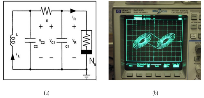
Figure 6 (a) Chua circuit. (b) Chua attractor on oscilloscope.
