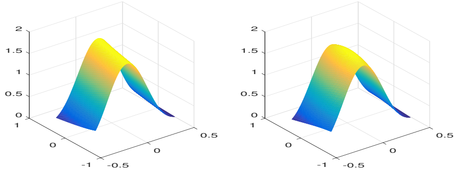
FIGURE 3. Example 2. Transition density (left) and the estimation (right). Selected dimensions (2,41), 100 \cdot \text{MISE} = 0.16 . N = 200 , T = 10 , \Delta = 0.01 , t = 1 .
