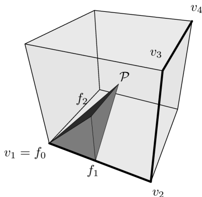
FIGURE 9. The characteristic simplex \Delta_{\Phi} (in dark gray) and the characteristic vertices V_{\Phi} = (v_1, v_2, v_3, v_4) with respect to the flag \Phi = (f_0, f_1, f_2, \mathcal{P}) of a cube.
