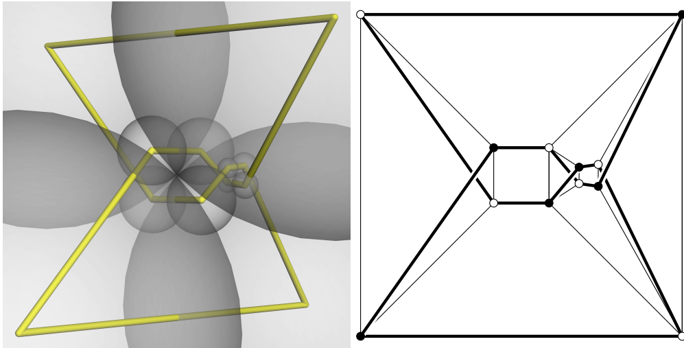
FIGURE 20. (Left) An orthocubic representation of the trefoil knot and its corresponding cubic diagram (right).
