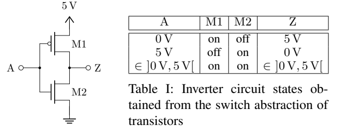
Fig. 3: Inverter circuit
