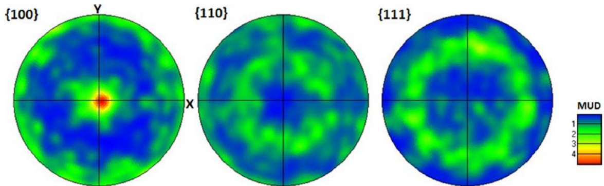
Figure 8: {100}, {110} and {111} pole figures corresponding to the (X-Y) plane of as-built 17-4 PH steel in figure 5 showing a \langle 100 \rangle preferred orientation of grains elongated in the build direction.
