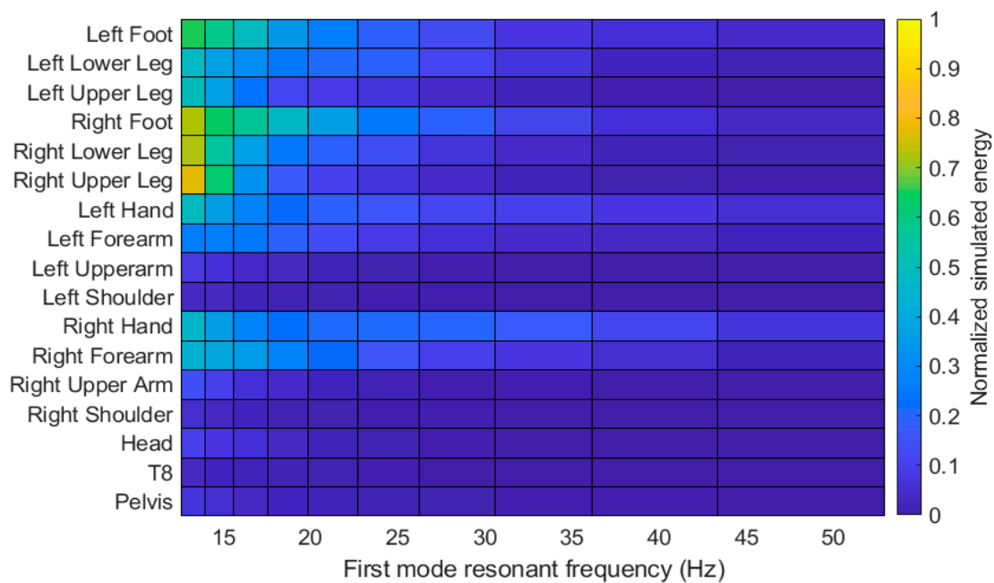
Figure 1. Normalized harvested energy on different body locations for a constant active material volume. Longer lengths and narrower widths correspond to lower resonance frequencies.
