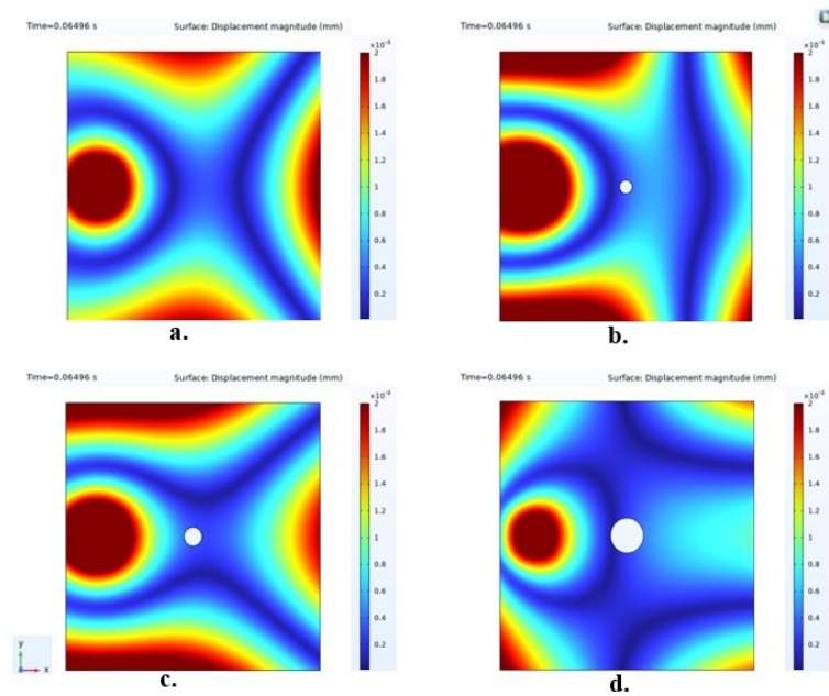
Figure 17. The surface plots of the analyzed sample cases displaying the displacement magnitude for visualization of the disturbance created by damage on the Lamb waves. In these representations, (a) illustrates the healthy structure in its intact state, (b) shows a structure with 5 mm hole damage, (c) demonstrates a structure with 7 mm hole damage, and (d) displays a structure with 13 mm hole damage.
