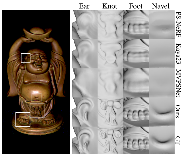
Figure 1. One image from DiLiGenT-MV’s Buddha dataset [13], and 3D reconstruction results from several recent MVPS methods: [12, 27, 28] and ours. The latter provides the fine details closest to the ground truth (GT), while being remarkably simpler.
