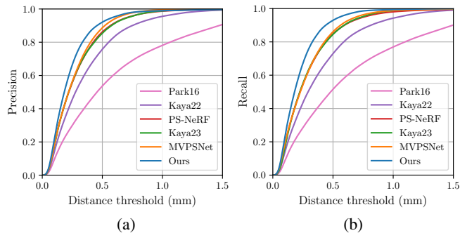
Figure 11. (a) Precision (higher is better) and (b) recall (higher is better) as functions of the distance error threshold, in comparison with other state-of-the-art methods.
