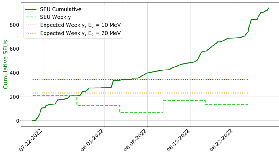
Fig. 4. In-flight SEU measurements as a function of time for the Cypress SRAM before the failure, cumulative, and weekly data. Expected weekly data are based on calculations in Tables IV for proton measurements with Weibull fit with mixed-shielding.
