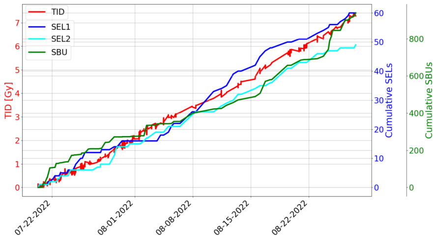
Fig. 6. In-flight TID, SEL, and SEU measurements as a function of time until August 27th, 2022.
