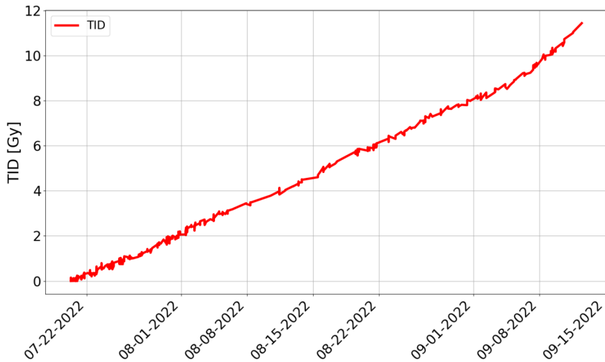
Fig. 5. In-flight TID measurements as a function of time for the whole mission duration.
