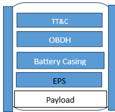
Fig. 2. Cartoon of the CELESTA CubeSat printed circuit board (PCB) stackup, including the telemetry, tracking and control (TT&C), on-board data handling (OBDH), electric power system (EPS), the battery, and the payload.
