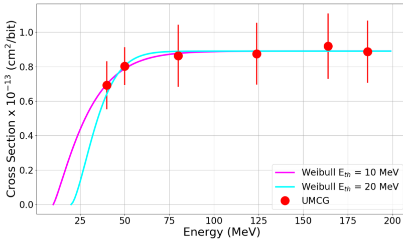
Fig. 8. Proton SEU cross section Weibull fits for the Cypress SRAM measured at UMCG.
