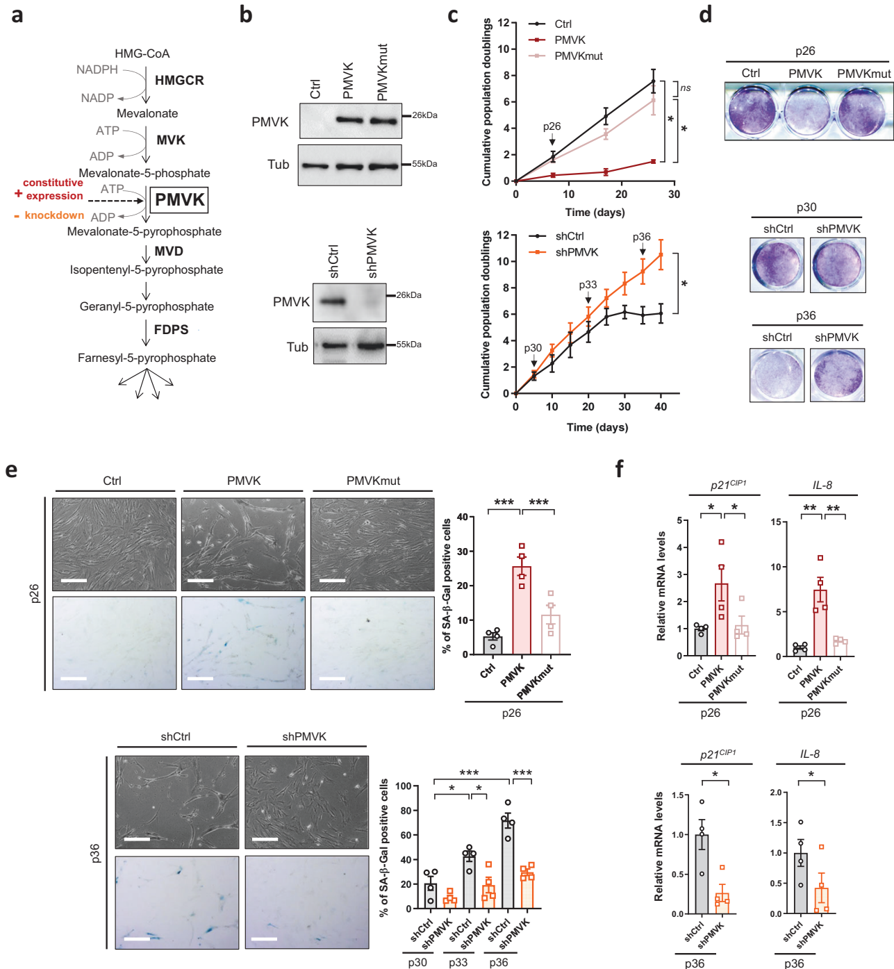
Fig. 1 The MVA pathway regulates cellular senescence in normal cells. a Schematic representation of the MVA pathway in eukaryotic cells. HMGCR, HMG-CoA reductase; MVK, mevalonate kinase; PMVK, phosphomevalonate kinase; MVD, mevalonate-diphosphate decarboxylase; FDPS, farnesyl diphosphate synthase. Constitutive expression (in red) or knockdown by shRNA (in orange) was performed in MRC5 fibroblasts. b Relative PMVK and Tubulin protein levels in empty vector (Ctrl), PMVK- or Kinase Dead (PMVKmut) PMVK-expressing cells and in shCtrl- or shPMVK-expressing cells. c Growth curves of Ctrl, PMVK- or PMVKmut-expressing cells, and shCtrl and shPMVK-expressing cells. Mean \pm SEM of n = 4 independent biological replicates. RM one-way ANOVA test on last time point. d Crystal violet staining of Ctrl, PMVK- or PMVKmut-expressing cells at early passage (p26), and of shCtrl- and shPMVK-expressing cells at early (p30) and late (p36) passage. e Micrographs and quantification of SA- \beta -gal positive cells of Ctrl, PMVK- or PMVKmut-expressing cells at early passage (p26), and of shCtrl- and shPMVK-expressing cells during passages. Mean \pm SEM of n = 4 independent biological replicates. Scale bar: 100 \mu m. RM one-way ANOVA test (upper panel) and paired Student's T-test (lower panel). f RT-qPCR of p21 CIP1 and IL-8 genes in Ctrl, PMVK- or PMVKmut-expressing cells at early passage (p26), and of shCtrl- and shPMVK-expressing cells at late passage (p36). Mean \pm SEM of n = 4 independent biological replicates. RM one-way ANOVA test (upper panel) and paired Student's T-test (lower panel). ns (nonsignificant; * p < 0.05 ; ** p < 0.01 ; *** p < 0.001 ).
