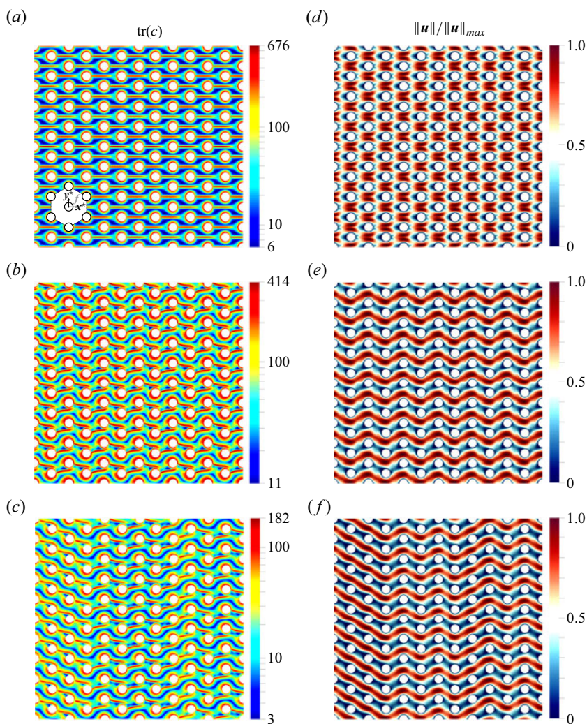
Figure 9. Examples of steady-state fields for \text{tr}(c) and the corresponding normalized amplitude of the velocity; (a) ( \beta = 0.5, Wi = 42 ) corresponds to the trivial steady solution, (b) ( \beta = 1, Wi = 53.2 ) to the regime (III) and (c) ( \beta = 5, Wi = 19.6 ) to regime (IV).
