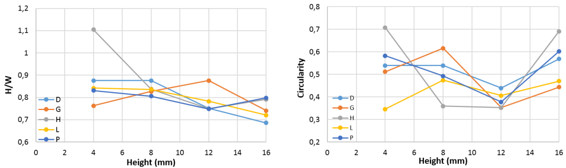
Figure 9: (Left) height/Width ratio VS height in Z, (right) circularity VS height in Z
