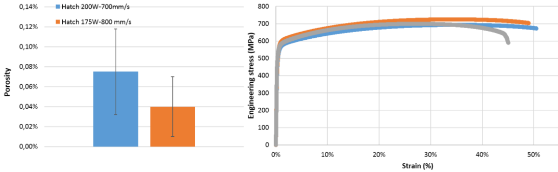
Figure 4: Porosity rates and tensile tests on 316L samples
