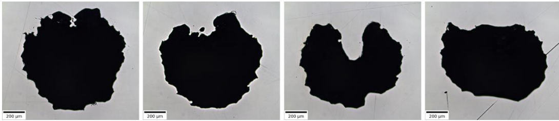
Figure 10: (From left to right) pores in Sample H, at 4, 8, 12 and 16 mm height
