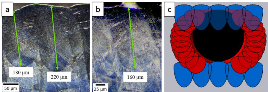
Figure 8: (a,b): hatching scan depth measured for a 200W and 700 mm/s parametrization. (c): X-Z Cross section of a schematic laser scans visualisation for a spherical pore of 300µm diameter with contour tracks(red) and hatching tracks (blue)
