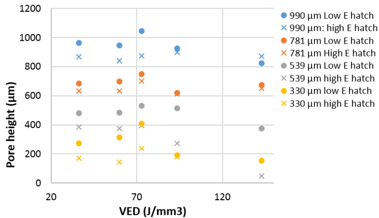
Figure 7: Pore height VS contour energy density for two different hatching energy densities (contour-hatching order)
