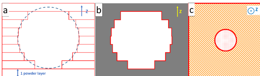
Figure 1: (a) X-Z slicing of a spherical pore in a CAD file, (b) resulting calculated contour inside the dense part, (c) X-Y view of one slice with the contour (red) and hatch (orange)
