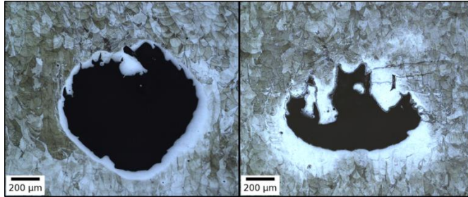
Figure 6: Etched sample C, 990 \mu\text{m} pore observed in an optical microscope in bright field for contour hatching (left) and hatching contour (right)
