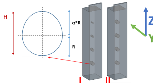
Figure 2: Samples fabricated by SLM and close-up on a pore section
