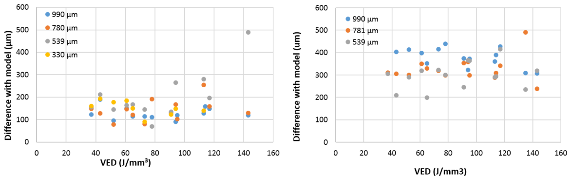
Figure 5: Difference in height with the CAD model (left) for contour-hatching (right) for hatching-contour
