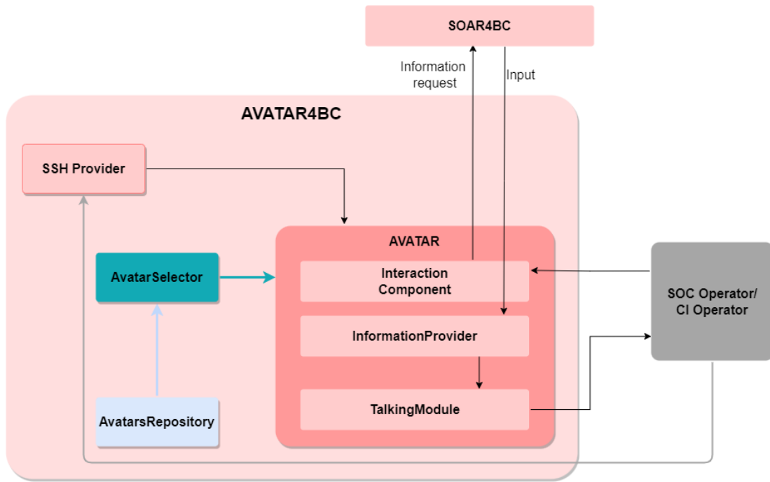
Fig. 2: AVATAR4BC architecture.
