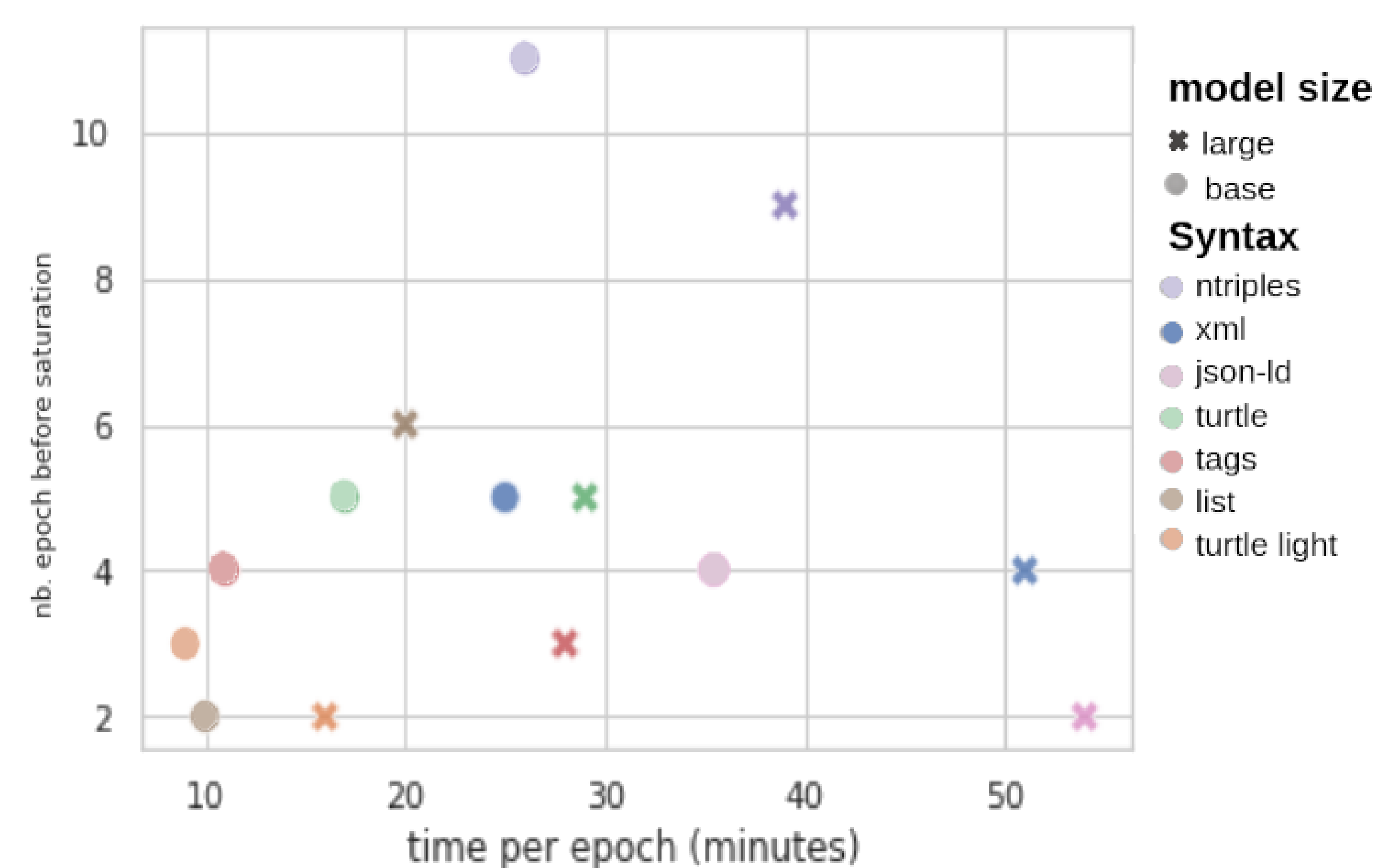
Figure 2. Number of epochs needed before reaching Micro-F1 saturation (> 0.9)
