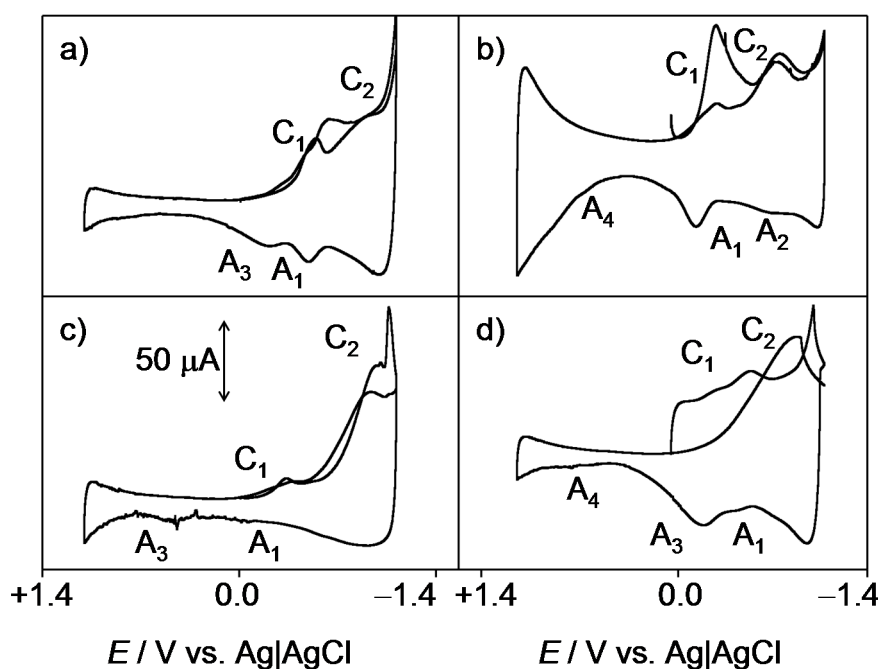
Figure 3. Cyclic voltammograms, after semi-derivative convolution, of (a) 2; (b) 3; (c) 4; and (d) 1 micro-particulate films on glassy carbon electrodes immersed into 0.10 M PBS at pH 7.4. Potential scan initiated at 0.0 V (a) in the negative and (b) in the positive directions; potential scan rate 50 \text{ mV}\cdot\text{s}^{-1} .
