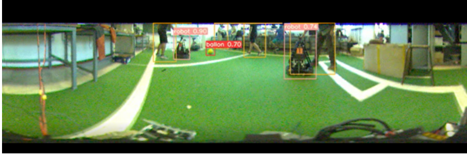
Fig. 1. YOLOv3 for object detection running on a GPU with omnidirectional camera.
