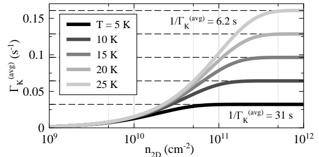
FIG. 8. Average Korrington-like relaxation rate \langle \Gamma_K \rangle as a function of 2D electron gas density at various temperatures in a 20-nm CdTe QW, calculated according to Eqs. (B10-B11). The relaxation time of a degenerate electron gas \tau_K^d is marked for T = 5 K and 25 K, highlighting the distinct \tau_K^d T = \text{const} behavior.
