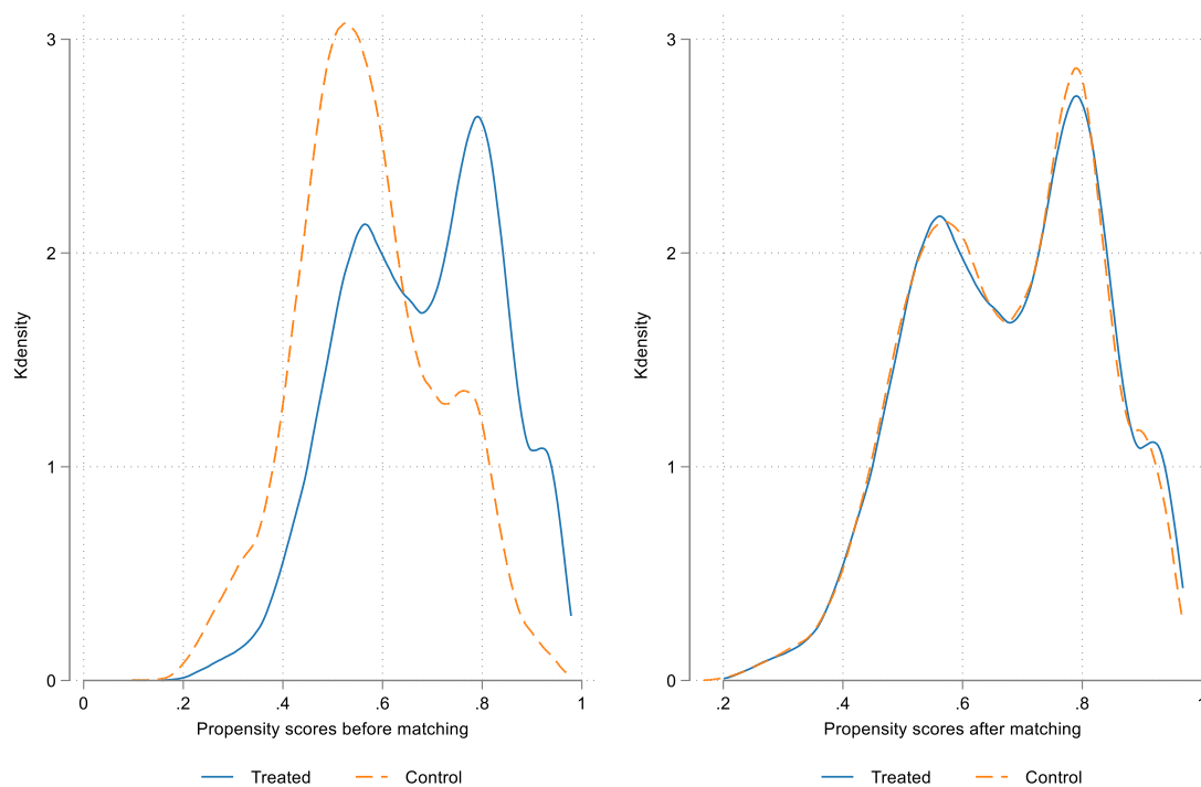
Figure A6: Propensity score before and after matching
