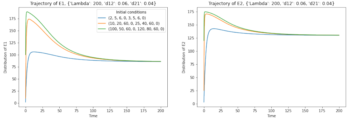
(b) \Lambda = 200 \text{ (day}^{-1}\text{)}
