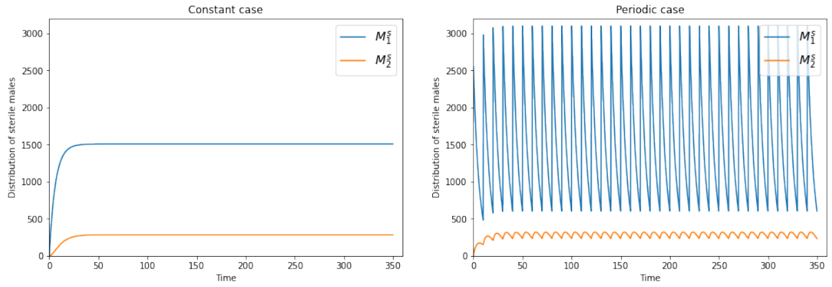
Figure 7: Densities of M_1^s and M_2^s in both cases. Left : constant continuous releases with \Lambda = \bar{\Lambda} = 250.88 \text{ (day}^{-1}\text{)} , Right : periodic impulsive releases with \Lambda^{\text{per}} = \bar{\Lambda}^{\text{per}} = 255.15 \text{ (day}^{-1}\text{)} .
