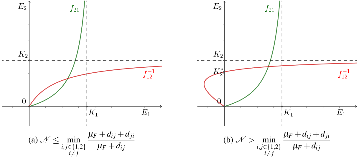
Figure 1: Behaviors of f_{21} and f_{12}^{-1}
