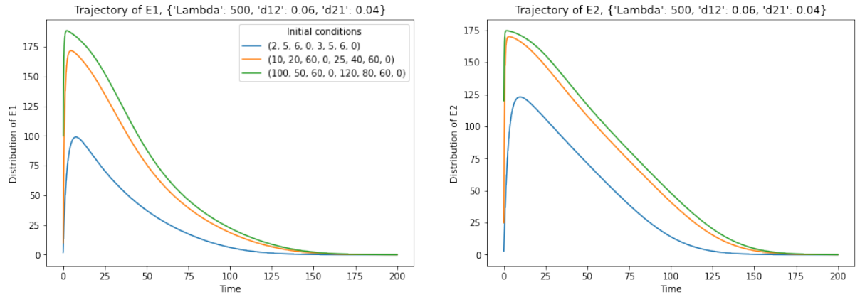
(c) \Lambda = 500 \text{ (day}^{-1}\text{)}
