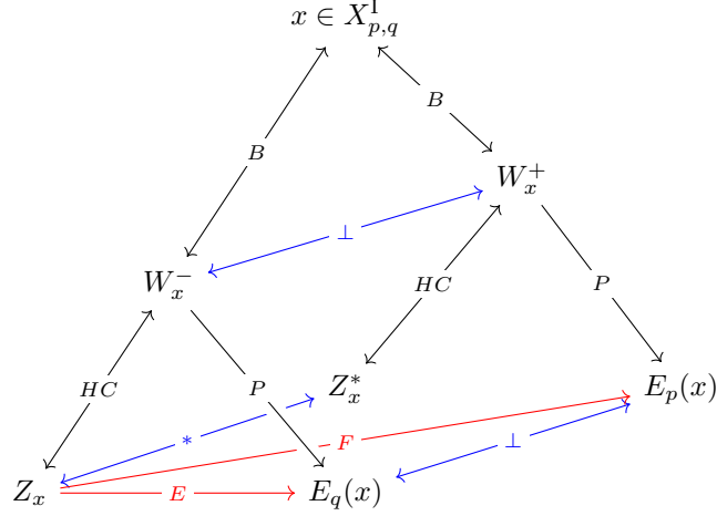
Figure 1: A synthetic view of the Borel and Harish-Chandra embeddings and the maps E and F (in red) for Type I.
