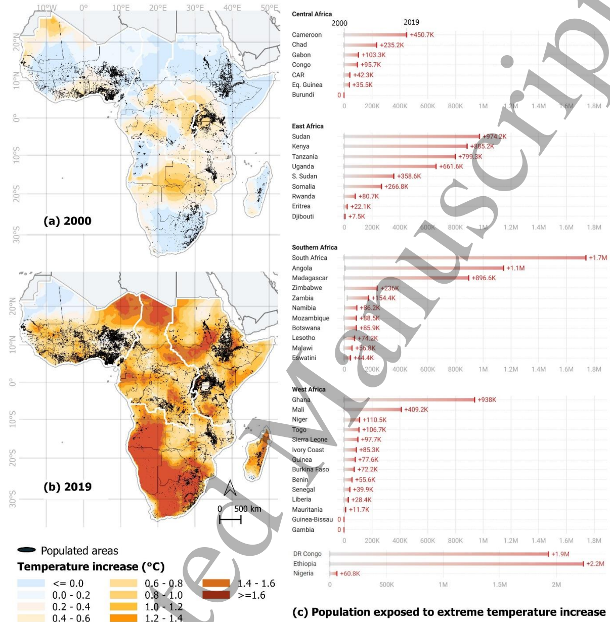
Figure 2 Temperature increase and population exposure. (a) spatial patterns of temperature increase (sky blue to orange) and populated areas (pixels with more than 100 persons) in 2000 (black); (b) spatial patterns of temperature increase and populated areas (pixels with more than 100 persons) in 2019; (c) country-wise levels of population exposed to extreme temperature increase ( > 1^\circ\text{C} increase in average annual temperature compared to the reference year -twenty years- before). The three most populated countries - DR Congo (Central Africa), Ethiopia (East Africa), and Nigeria (West Africa) - are presented on a separate scale.
