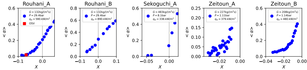
Figure 1: Examples of (X, < \alpha >) plots found in the literature that we use to determine the point of OSV. The red marker in the first plot represents the identified point of OSV. Series without markers are disqualified for different reasons. Each run condition is given in the legend of the figure. Water is used in every one. Rouhani_A&B : Data from Rouhani (1966a). Rouhani_B is disqualified as we do not have enough points at low void fraction to see the inflection in (X, < \alpha >) . Sekoguchi_A : Data from Sekoguchi et al. (1980). This run isn't considered as it does not have enough datapoints. Zeitoun_A&B : Data from Zeitoun (1994). Data in run Zeitoun_A is too irregular. In Zeitoun_B < \alpha > \sim 10\% at the inflection, proposed at X = -0.022 by the author. We find this too high for an OSV criterion.
