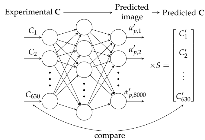
Figure 12. Training strategy using a training database with only experimental data.
