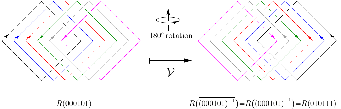
FIGURE 8. If we apply the isotopy \mathcal{V} to the ring link R(000101) we obtain the ring link R(\overline{(\overline{000101})^{-1}}) = R(010111) . The permutation of this R(000101) \mapsto R(010111) isotopy is the reverse permutation \nu on [6]. In general, if we apply \mathcal{V} to a ring link R(a) we obtain the ring link R(\bar{a}^{-1}) , that is, \mathcal{V} \mid R(a) \rightarrow R(\bar{a}^{-1}) . If R(a) has n components then \mathcal{V} maps the i -th component of R(a) to the (n - i + 1) -st component of R(\bar{a}^{-1}) , for i = 1, \dots, n . That is, \mathcal{V} \mid R(a) \xrightarrow{\nu} R(\bar{a}^{-1}) .
