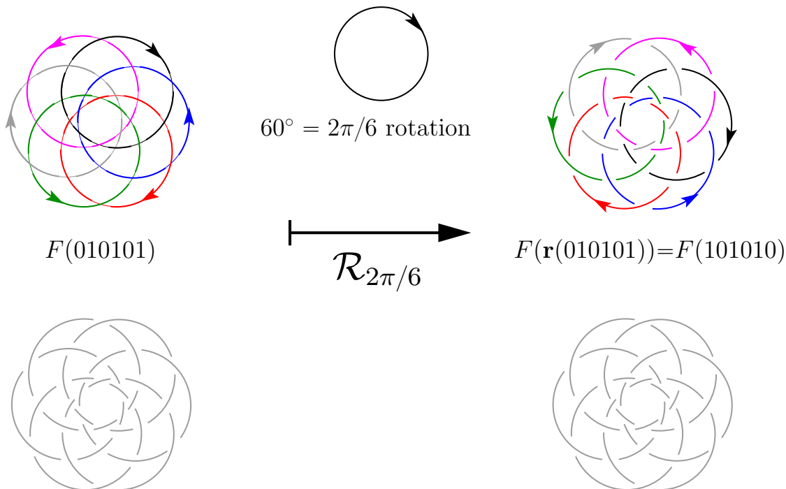
FIGURE 17. The isotopy \mathcal{R}_{2\pi/6} takes F(010101) to F(101010) . If we ignore the orientations of the components, as we do at the bottom of this figure, we realize that this isotopy actually takes F(010101) to itself. Thus it is valid to say that this isotopy takes F(010101) to itself, but with the i -th component of F(010101) taken to the (i \oplus_6 1) -st component of F(010101) with its orientation reversed. Thus this isotopy witnesses that (1, -1, -1, -1, -1, -1, \sigma) is an intrinsic symmetry of F(010101) .
