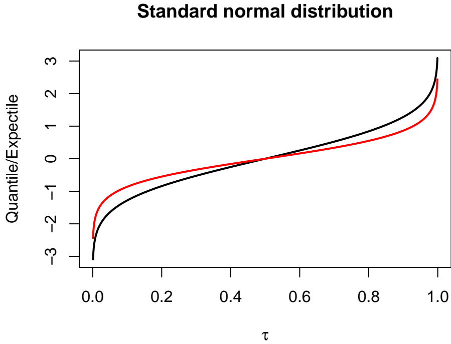
Figure C.1: Quantiles (black) and expectiles (red) of the standard Gaussian distribution, as functions of \tau \in (0, 1) .
