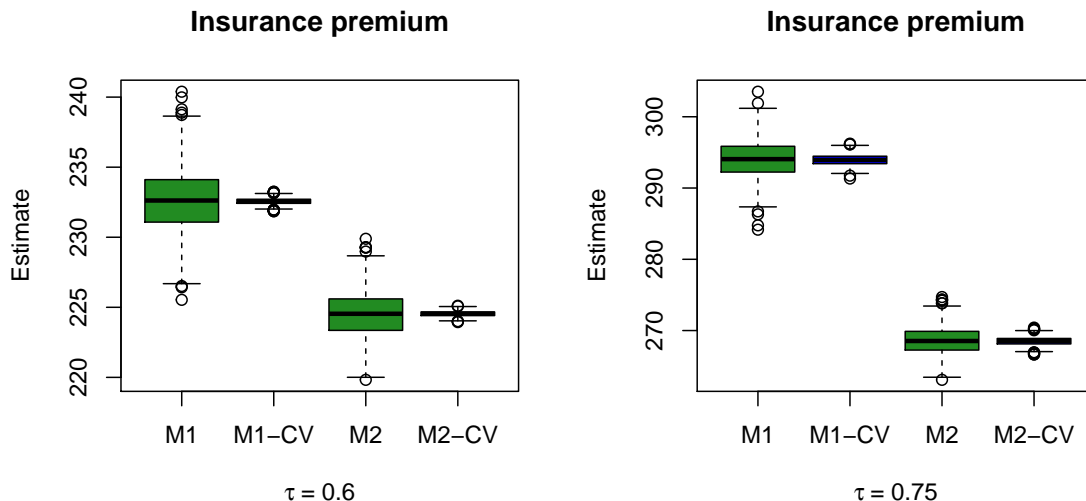
Figure 4: Insurance premium example. Boxplots of \hat{\xi}_{\tau,n} (green) and \tilde{\xi}_{\tau,n} (blue) for \tau = 0.6 (left) and \tau = 0.75 (right). In model 1 we let the X_i have an exponential distribution with mean 100, and in model 2 we let the X_i have a Pareto distribution with extreme value index \gamma = 1/4 , rescaled to have mean 100. In both models, T = 20 and \lambda = 0.1 , and 1,000 Monte-Carlo replications of an independent sample of size n = 10,000 were used.
