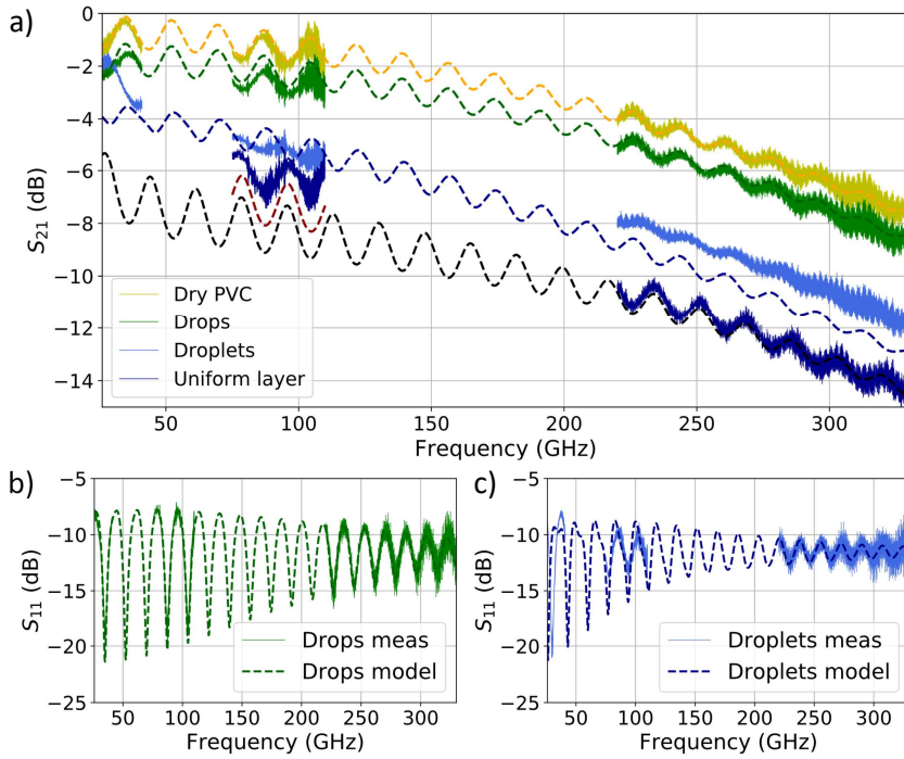
Fig. 7 a) Measured transmitted magnitude through a radome covered by water under different shapes in the Ka, W and J bands. Dashed-lines : the model given by (4) applied for the different values of \alpha (share of wet surface). Measured reflected magnitude towards dry side compared with the model for the b) drops and c) droplets water shapes.
