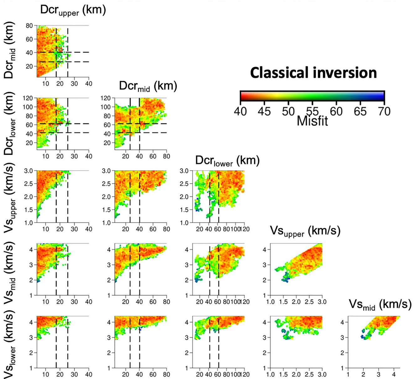
Figure F1. Correlations between the depth and the S-wave velocity of the three crustal layers, for all the models accepted by the classical inversion. D_{cr\_upper} , D_{cr\_mid} , D_{cr\_lower} , and V_{S\_upper} , V_{S\_mid} , V_{S\_lower} , refer to the depths and V_S of the upper, mid, and lower crusts, respectively. Red and blue colors indicate small and large misfit values, respectively. The black dashed lines are the allowed depth range for D_{cr\_upper} , D_{cr\_mid} , and D_{cr\_lower} , used in Section 5.4.
