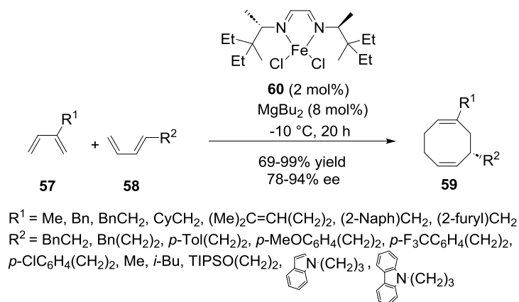
Scheme 19. [4+4] Cycloaddition of 1,3-dienes.
