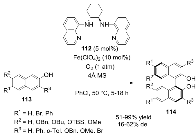
Scheme 32. Oxidative coupling reaction of 2-naphthols.
