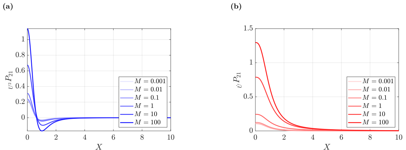
FIG. 7: First-order pressure correction P_{21} in the top layer as a function of horizontal coordinate X , as obtained from numerically solving Eqs. (47,48) with \alpha = 15 , \beta = 99 , and \text{Bo} = 0.01 , and for various M as indicated. Both the lift term U^2P_{21} (a) with V_1 = 0 and V_2 = 1 , and inertial term \dot{U}P_{21} (b) with \dot{V}_1 = 0 and \dot{V}_2 = 1 , are shown.
