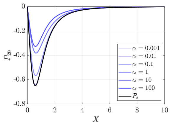
FIG. 3: Zeroth-order excess pressure fields, P_{10} (a) and P_{20} (b), as functions of the horizontal coordinate X , as evaluated from Eqs. (32,33) for M = 2 and \beta = 99 , with V_1 = 1 and V_2 = 1 , and different values of \alpha as indicated. The black line in panel (a) represents the top-layer pressure field for \alpha = 0.001 , with the appropriate scale on the right y -axis. The black line in panel (b) represents the pressure profile P_s generated near a solid boundary [10].
