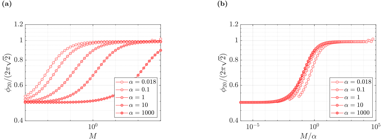
FIG. 11: (a) Coefficient \phi_{20} of the zeroth-order torque per unit length (see Eq. (??)) exerted on the top cylinder, and normalized by the value for a rigid no-slip boundary, as a function of the viscosity ratio M and for various gap ratios \alpha . This coefficient was computed for \beta = 99 , V_1 = 0 , and V_2 = 1 . (b) Same data with a rescaled parameter M/\alpha on the x -axis.
