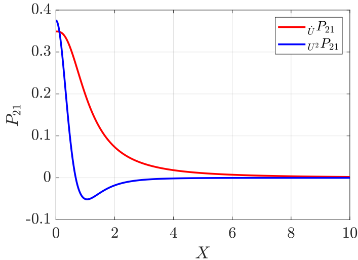
FIG. 6: First-order pressure correction P_{21} in the top layer as a function of horizontal coordinate X , as obtained from numerically solving Eqs. (47,48) for M = 2 , \alpha = 15 , \beta = 99 , and \text{Bo} = 0.01 . Both the lift term U^2P_{21} (blue) for V_1 = 0 and V_2 = 1 , and inertial term \dot{U}P_{21} (red) for \dot{V}_1 = 0 and \dot{V}_2 = 1 , are shown.
