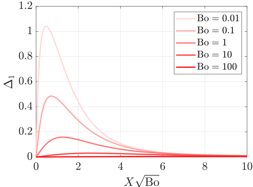
FIG. 4: First-order interface deflection profile \Delta_1 as a function of rescaled horizontal coordinate X\sqrt{\text{Bo}} , as calculated from Eq. (35) with M = 2 , \alpha = 15 , \beta = 99 , V_1 = 0 , V_2 = 1 , and for several Bo values as indicated.
