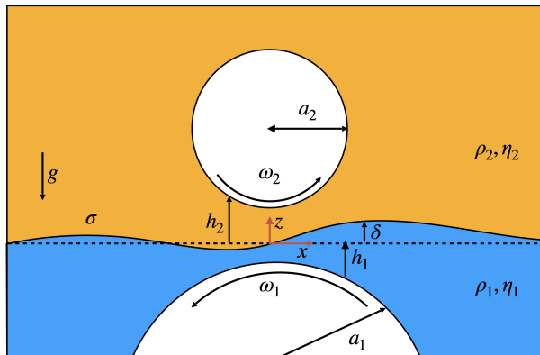
FIG. 1: Schematic of the system. Two rigid infinite cylinders rotate with prescribed velocities near a capillary interface between two incompressible Newtonian viscous fluids. The origin of spatial coordinates is located at the undeformed fluid interface ( z = 0 ) in the line joining the centers of mass of the cylinders ( x = 0 ). The deformed fluid interface is located at z = \delta(x, t) .
