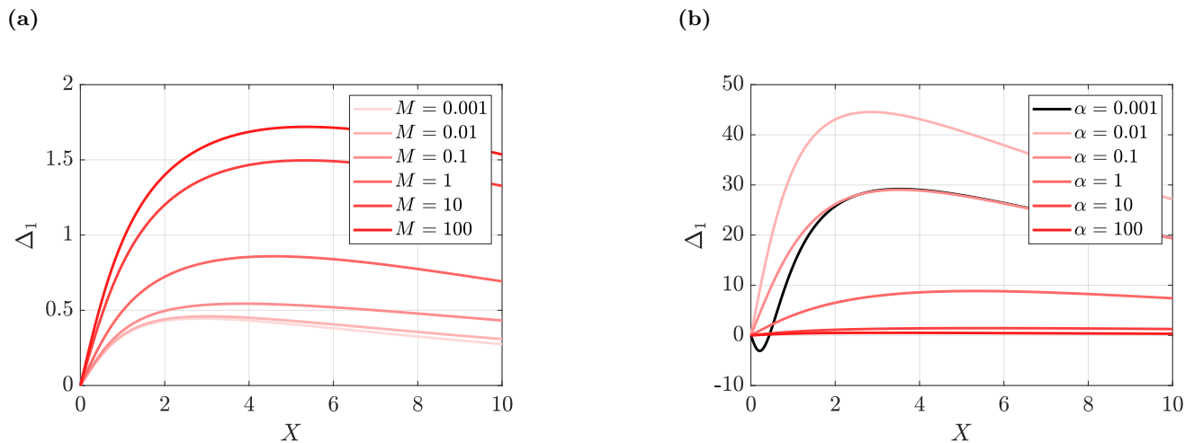
FIG. 5: First-order interface deflection profile \Delta_1 as a function of horizontal coordinate X , as calculated from Eq. (35) with \text{Bo} = 0.01 , \beta = 99 , V_1 = 0 and V_2 = 1 , for: (a) \alpha = 15 and varying M as indicated; and (b) M = 2 and varying \alpha as indicated.
