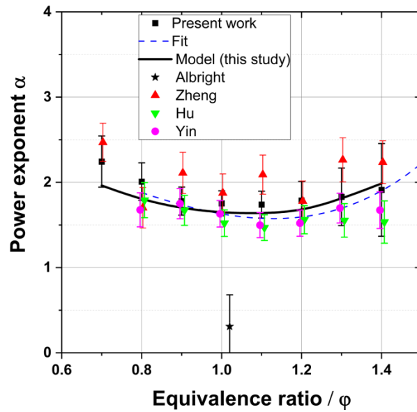
Fig. 20. Power exponent \alpha of DIB/air flames at atmospheric pressure. –Symbols: present measurements, solid line: predictions of the present kinetic model, dashed line – empirical expression [14].
