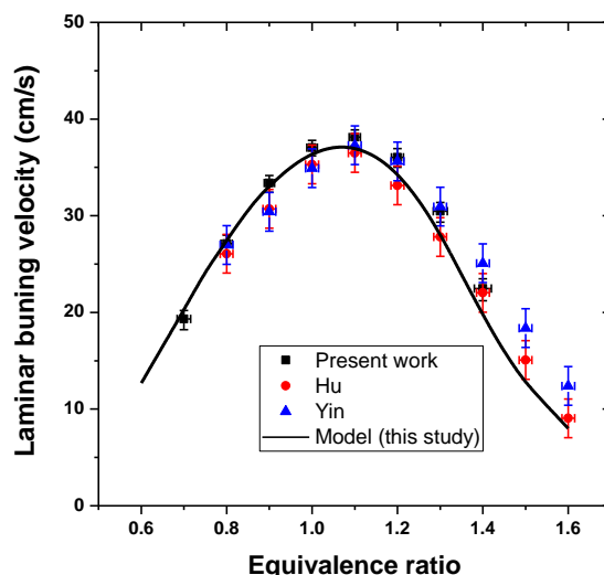
Fig. 16. Laminar burning velocity of DIB/air flames at 1 atm and initial temperature of 298 K. Symbols: experiments, line: modeling. Squares: DIB/air, present study, circles: DIB-1/air [14], triangles: DIB-2/air [15].
