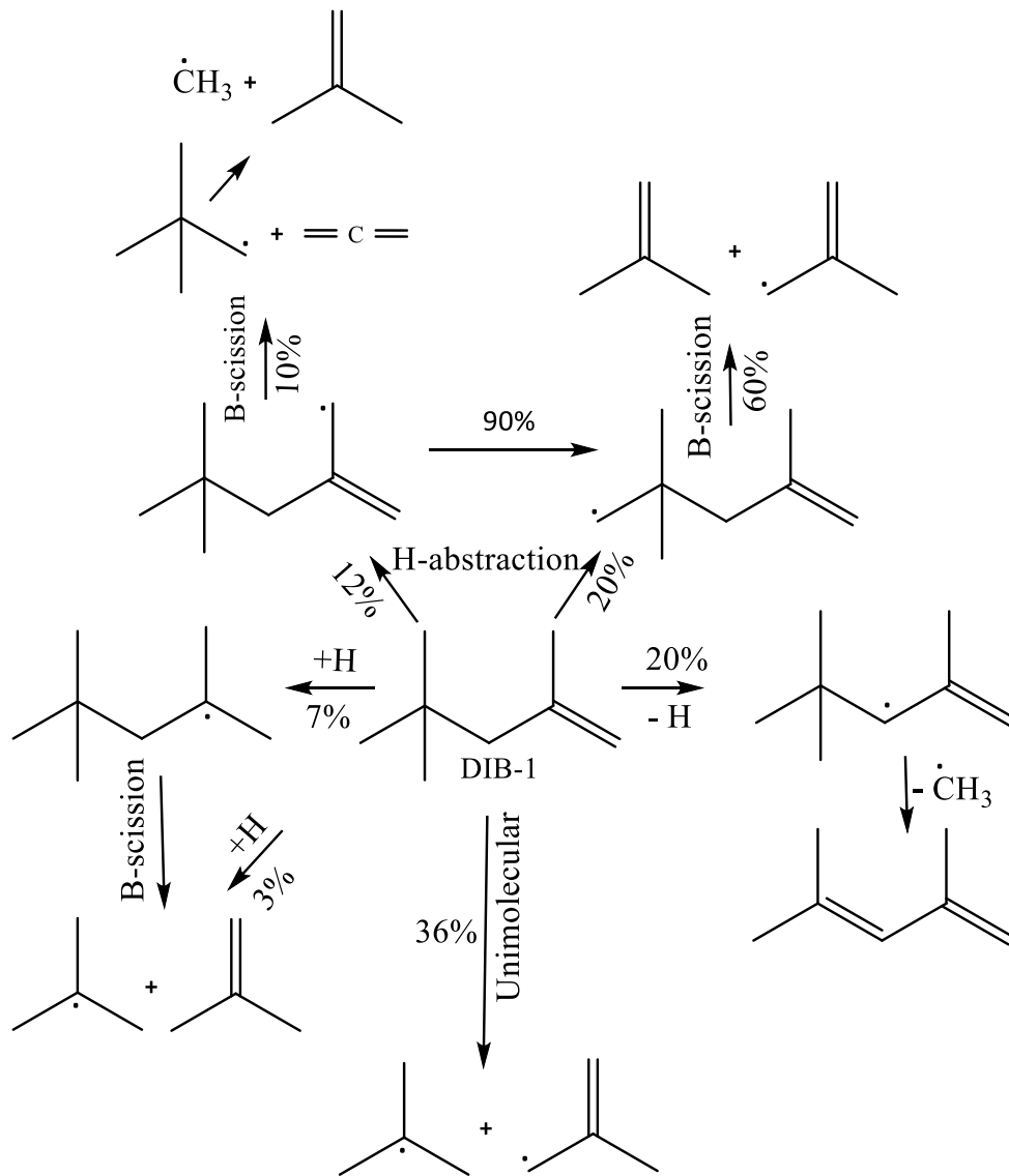
Fig. 14. Flux analysis using the current model for DIB-1 at \phi = 1.0 in air, 30 bar at 1200 K and 20% fuel consumption, proceeds via various pathways producing isobutene and/or its related radicals.
