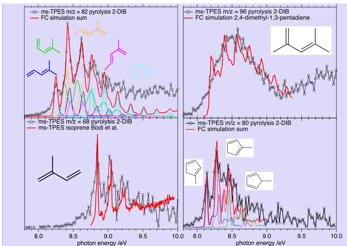
Fig. 7. Photoion mass-selected threshold photoelectron spectra of larger species appearing during the decomposition of DIB-2, as measured in a 1150—1500 K reactor temperature range. Reference spectra from [25] and [55].
