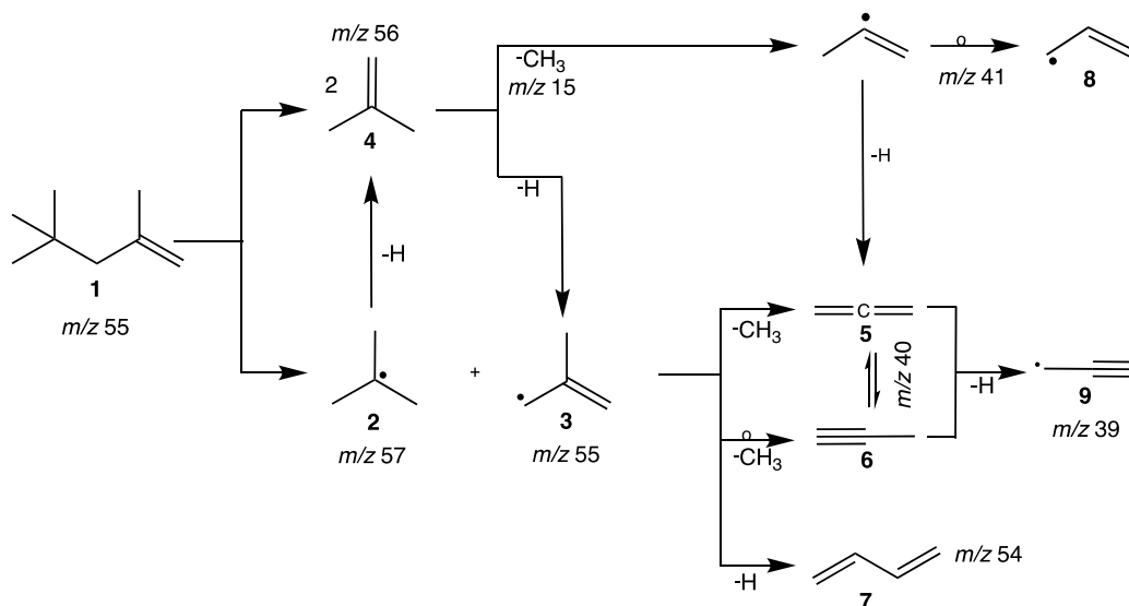
Fig. 4. Reaction mechanisms of the DIB-1 decomposition at unimolecular pyrolytic conditions.
