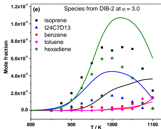
Fig. 10. Flow reactor analysis at \phi = 3.0 and 0.85 atm with a residence time of 0.22_s for (a) the consumption of DIB isomers and formation of isobutene from both isomers, (b) formation of C_1 – C_3 species from DIB-1, and (c) other major products formed from DIB-1, (d) formation of C_1 – C_3 species from DIB-2, and (e) other major products formed from DIB-2, across the temperature range of 800–1125 K.
