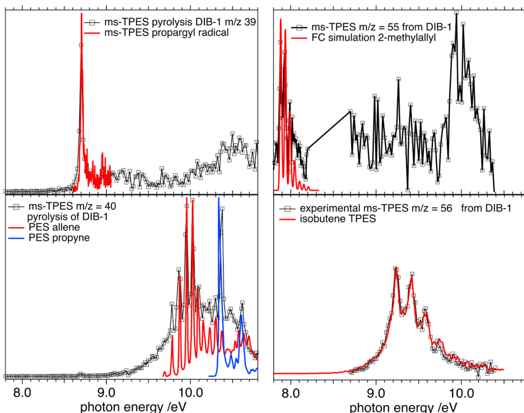
Fig. 3. Photoion mass-selected threshold photoelectron spectra (ms-TPES) of the intermediates and reaction products in the temperature range at 975—1175 K . PES is photoelectron spectra from the literature. Species are isomer-selectively assigned using either Franck—Condon (FC) simulation or reference data (solid lines).
