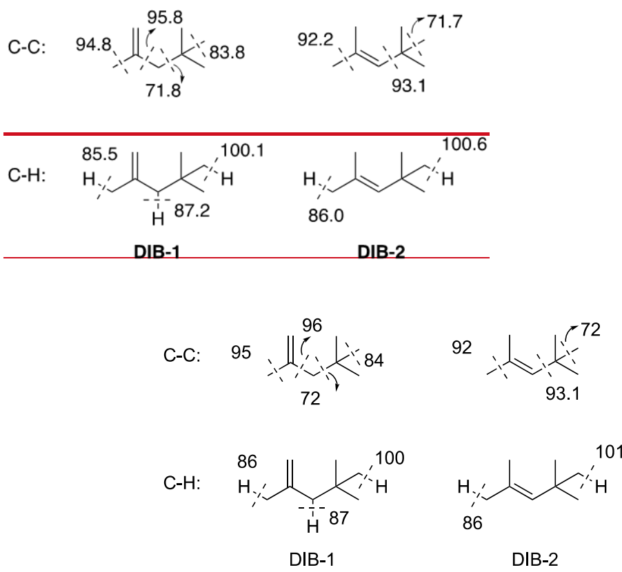
Fig. 1. Carbon–carbon and carbon–hydrogen bond dissociation enthalpies (BDE, in kcal mol -1 ) computed using the G4 composite theory at 298K. Dashed lines indicate bond dissociation.
