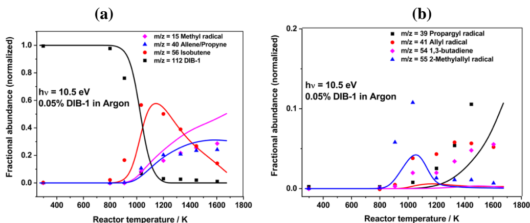
Fig 2. Semi-quantitative temperature dependent species profiles measured during the thermal decomposition of DIB-1. Symbols: experiment, lines: modeling model from this study assuming constant pressure and residence time of 15 mbar and 50 \mu s respectively covering temperatures from 300 – 1800 K. The fractional abundance is normalized based on the initial fuel concentration (see Table S3).
