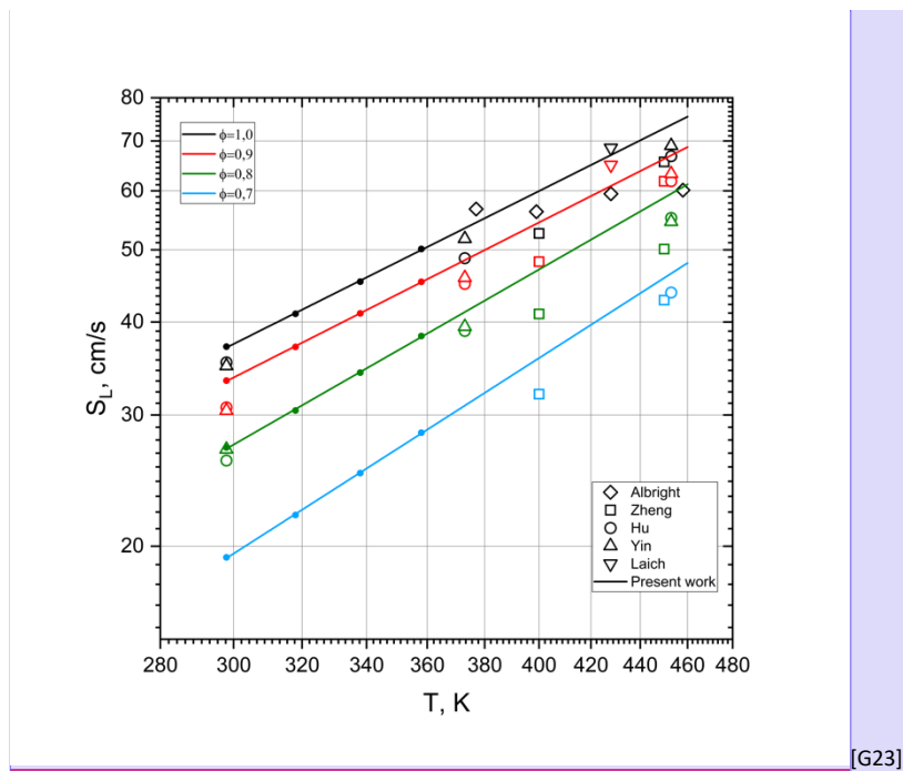
Fig. 18. Laminar burning velocity of lean and stoichiometric DIB/air flames at 1 atm and different initial temperatures. Symbols: experimental data, lines: trendlines based on the present measurements (solid symbols).
