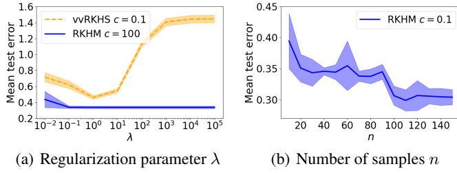
Figure 4: Mean test error versus hyperparameters (Mean value \pm standard deviation of 5 runs).
