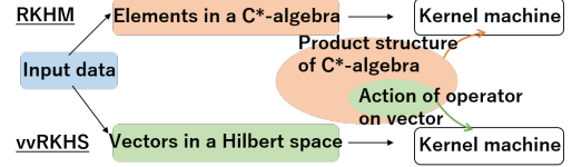
Figure 3: Comparison of RKHM with vvrKHS
