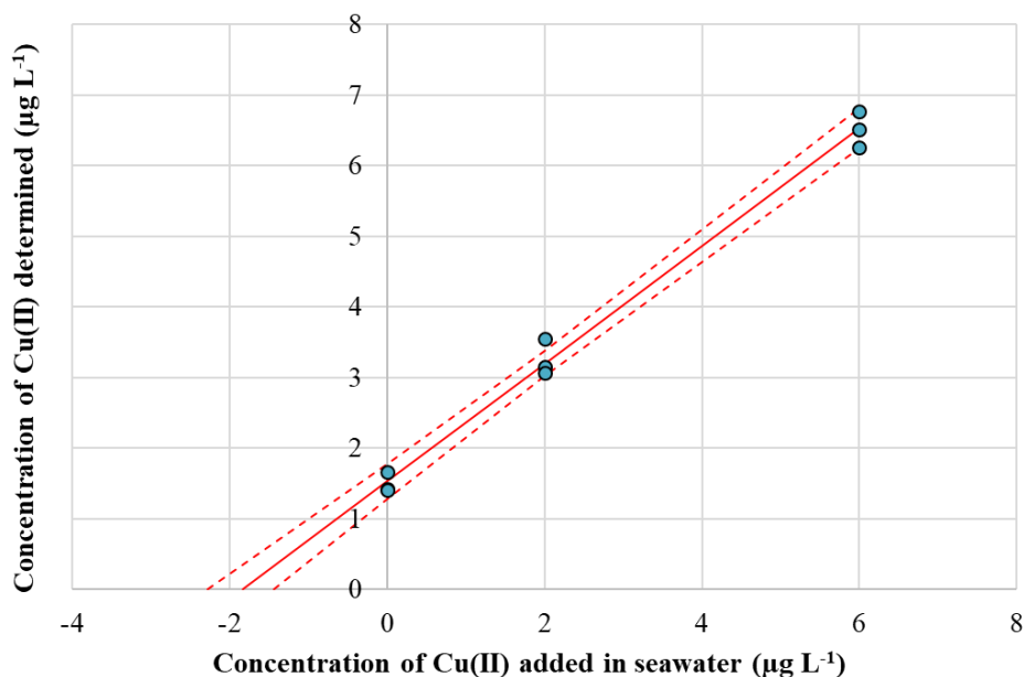
Figure 5 Determination of Cu(II) concentration in seawater by means of standard addition method. The dotted hyperbolic curves were obtained with a confidence interval of 95%. The experiments were conducted in triplicate for each concentration level.
