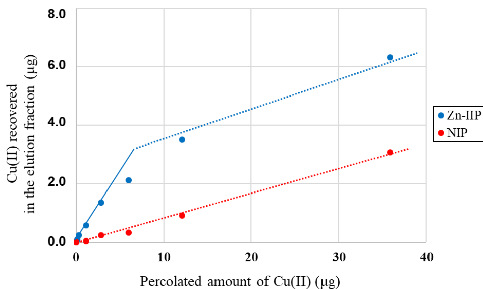
Figure 4 Adsorption capacity curves obtained by percolating an increasing amount of Cu(II) in 1 mL of HNO 3 at pH 5.5 on Zn-IIP and its NIP (30 mg for each). Amounts of Cu(II) were recovered in the elution fraction (1 mL of 5% HNO 3 ) after a washing step with 1 mL of Tris at 0.2 mM followed by 1.5 mL of HNO 3 at pH 3.6 and determined with ICP-MS.
