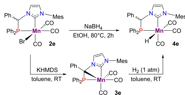
Scheme 4. Cooperative dihydrogen activation by NHC-phosphinomethanide complex 3e generated by deprotonation of Mn(I) NHC-phosphine precursor 2e .
