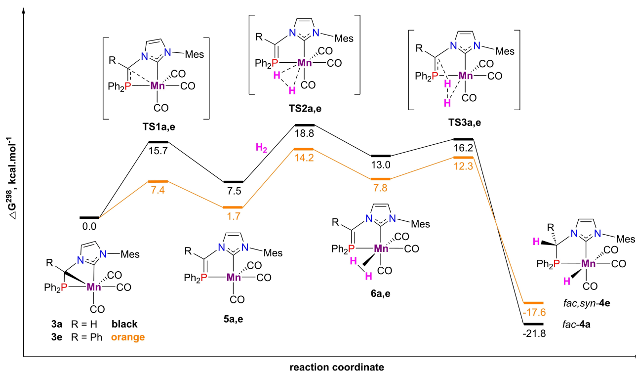
Scheme 5. The comparison of Gibbs energy profiles for cooperative dihydrogen activation with Mn(I) NHC-phosfinomethanide complexes 3a (R=H) [19] and 3e (R=Ph) at BP86/def2TZVP calculation level using toluene as SMD model (values are given in kcal.mol -1 and referred to 3a or 3e for each profile). Transition state TS2e was localized using slightly simplified model with a phenyl substituent at the NHC moiety.
