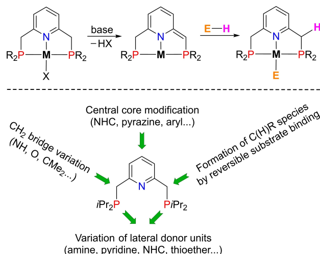
Scheme 1. Activation of inert bonds by metal-ligand cooperation via dearomatization of the central pyridine fragment in transition metal PNP pincer complexes (top) and structural modifications of this ligand scaffold (bottom).
